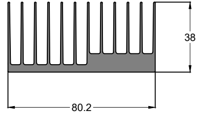
SEC. NO. IS00159 WEIGHT - 3.10 Kg/M
