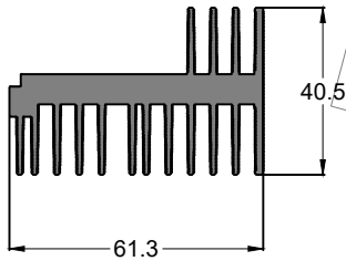
SEC.NO. IS00118 WEIGHT - 4.00 Kg/M
