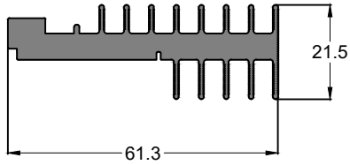
SEC. NO. IS00123 WEIGHT - 1.30 Kg/M
