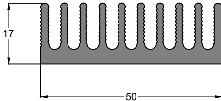
SEC. NO. IS0064 WEIGHT - 1.20 Kg/M
