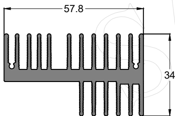
SEC. NO. IS0046
