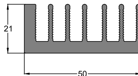
SEC. NO. IS00202 WEIGHT - 1.33 Kg/M
