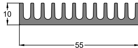
SEC. NO. IS00202 WEIGHT - 1.33 Kg/M
