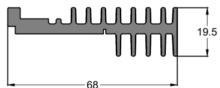
SEC. NO. IS00113 WEIGHT - 1.320 Kg/M
