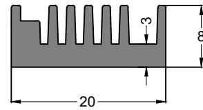
SEC. NO. IS00115 WEIGHT - 0.290 Kg/M
