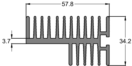
SEC. NO. IS0022
