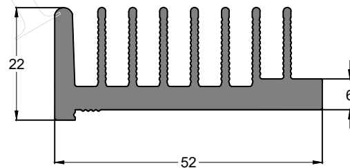
SEC. NO. IS0058
