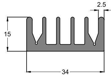
SEC. NO. IS0026
