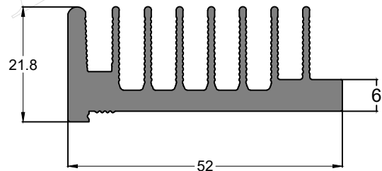
SEC. NO. IS00122 WEIGHT - 0.980 Kg/M
