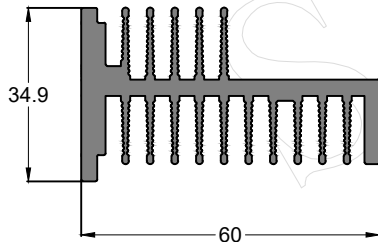
SEC. NO. IS00189 WEIGHT - 0.503 Kg/M
