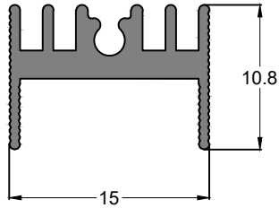
SEC. NO. IS00116 WEIGHT - 2.30 Kg/M
