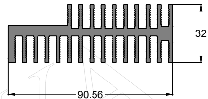
SEC. NO. IS00159 WEIGHT - 3.10 Kg/M
