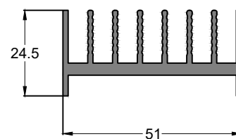
SEC. NO. IS00122 WEIGHT - 0.980 Kg/M
