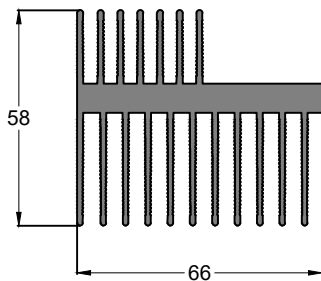
SEC. NO. IS00160 WEIGHT - 1.71 Kg/M
