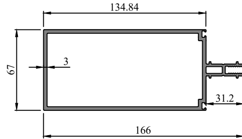
Profile Code - 272025 Weight KG /M - 3.602
