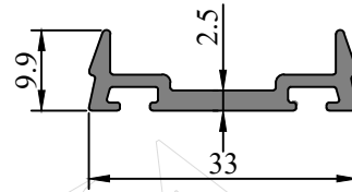
Profile Code - 366185 Weight KG /M - 0.286
