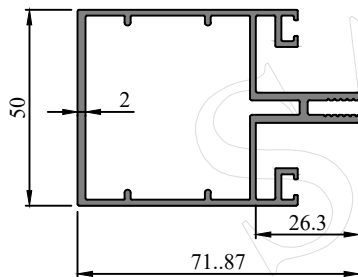
Profile Code - 272042 Weight KG /M - 1.335
