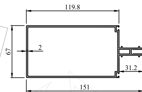
Profile Code - 272027 Weight KG /M - 2.561
