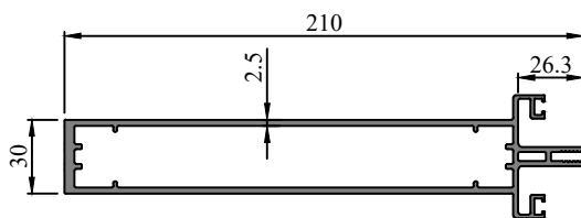
Profile Code - 272044 Weight KG /M - 3.600
