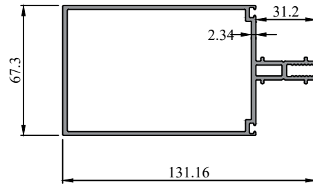
Profile Code - 272020 Weight KG /M - 2.30
