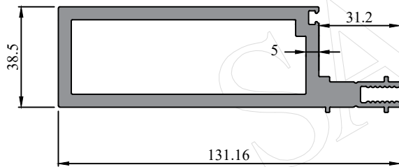
Profile Code - 273014 Weight KG /M - 4.10
