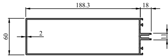
Profile Code - 272056 Weight KG /M - 3.036
