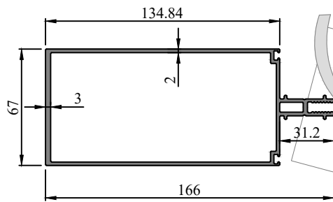
Profile Code - 272026 Weight KG /M - 2.736
