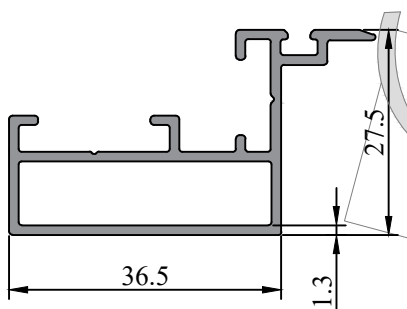
Profile Code - 541010 Weight KG /M - 0.520
