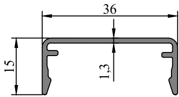
Profile Code - 366182 Weight KG /M - 0.331
