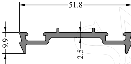
Profile Code - 366184 Weight KG /M - 0.252
