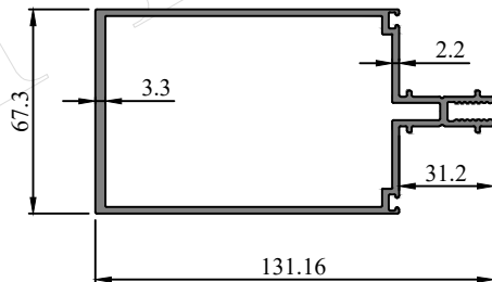
Profile Code - 272023 Weight KG /M - 2.51
