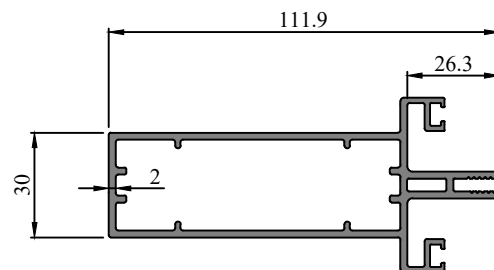
Profile Code - 272043 Weight KG /M - 2.422
