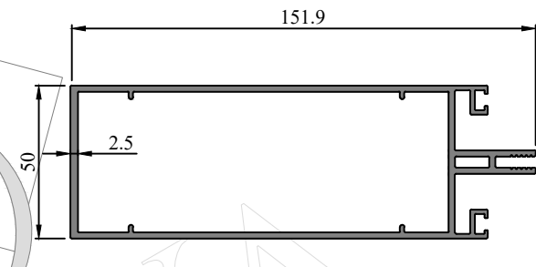
Profile Code - 272033 Weight KG /M - 2.562
