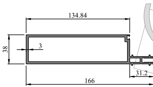
Profile Code - 273016 Weight KG /M - 3.119
