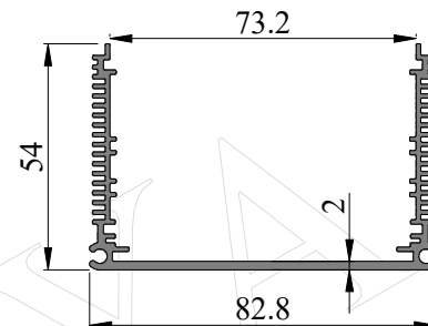
SEC. NO. IS00271 WEIGHT - 1.191 Kg/M
