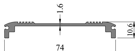
SEC. NO. IS0039 WEIGHT - 0.540 Kg/M
