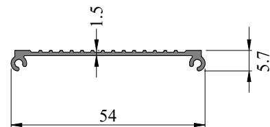
SEC. NO. IS0008 WEIGHT - 0.215 Kg/M
