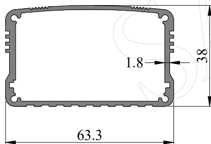
SEC. NO. IS00153 WEIGHT - 0.110 Kg/M
