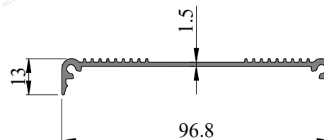
SEC. NO. IS00296 WEIGHT - 0.588 Kg/M
