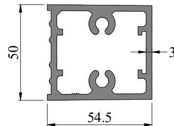
SEC. NO. IS0033 WEIGHT - 0.470 Kg/M
