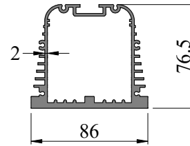
SEC. NO. IS0056 WEIGHT - 1.20 Kg/M
