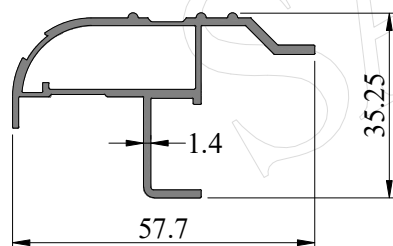
SEC. NO. IS0038 WEIGHT - 1.40 Kg/M
