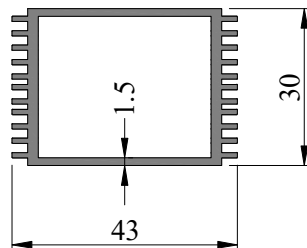
SEC. NO. IS0055 WEIGHT - 0.770 Kg/M
