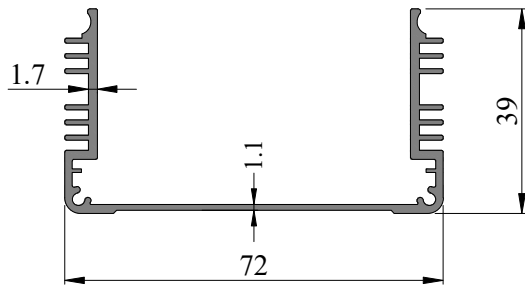
SEC. NO. IS00130R2 WEIGHT - 1.0 Kg/M
