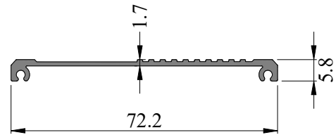
SEC. NO. IS00126 WEIGHT - 0.330 Kg/M
