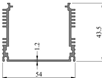
SEC. NO. IS0007 WEIGHT - 0.730 Kg/M
