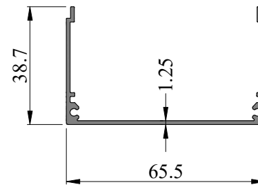
SEC. NO. IS00221 WEIGHT - 0.570 Kg/M
