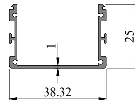
SEC. NO. IS00152 WEIGHT - 0.330 Kg/M
