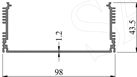
SEC. NO. IS0007 WEIGHT - 0.730 Kg/M
