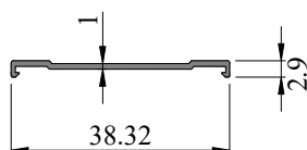
SEC. NO. IS00153 WEIGHT - 0.110 Kg/M
