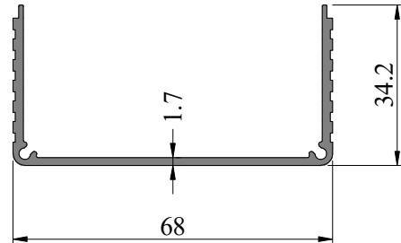
SEC. NO. IS0002 WEIGHT - 0.640 Kg/M
