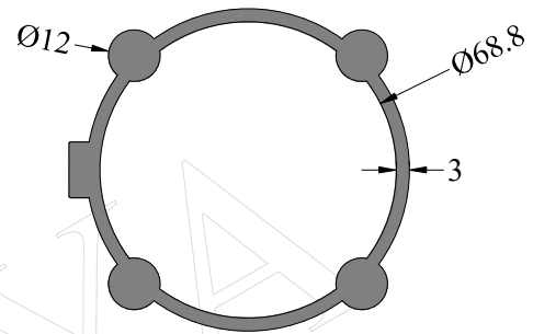
SEC.NO. IS0004 WEIGHT - 2.80 Kg/M
