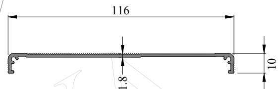
SEC. NO. IS00131R2 WEIGHT - 0.570 Kg/M
