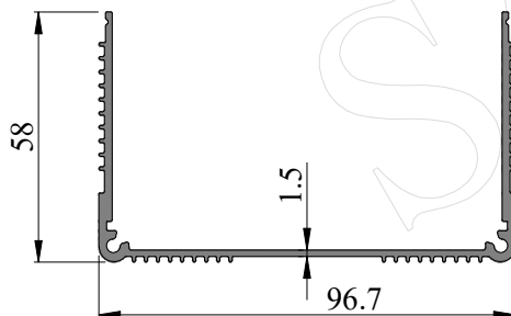
SEC. NO. IS00295 WEIGHT - 1.123 Kg/M
