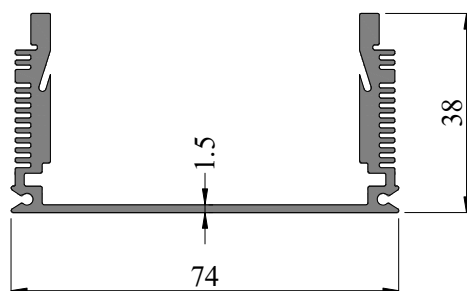
SEC. NO. IS0038 WEIGHT - 1.40 Kg/M
