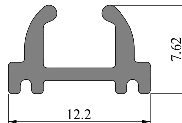
SEC. NO. IS0039 WEIGHT - 0.540 Kg/M
