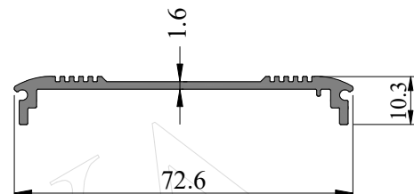
SEC. NO. IS0033 WEIGHT - 0.470 Kg/M
