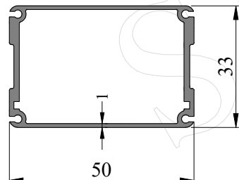
SEC. NO. IS0057 WEIGHT - 0.610 Kg/M
