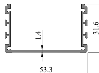
SEC. NO. IS00154R1 WEIGHT - 0.500 Kg/M
