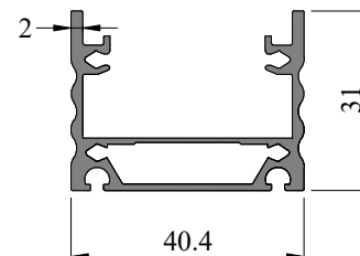
SEC. NO. IS0066 WEIGHT - 0.610 Kg/M
