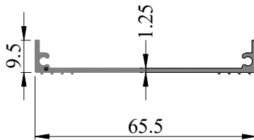
SEC. NO. IS00222 WEIGHT - 0.317 Kg/M
