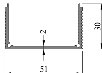
SEC. NO. IS0068 WEIGHT - 0.590 Kg/M
