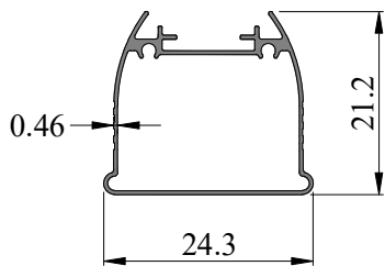
SEC. NO. IS0032 WEIGHT - 0.780 Kg/M
