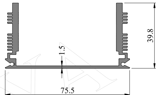
SEC. NO. IS0066 WEIGHT - 0.610 Kg/M
