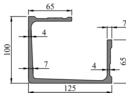
SEC. NO. FW0028 WEIGHT - 6.160 Kg/M
