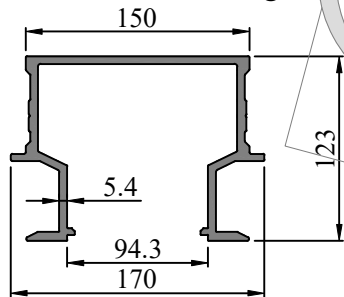
SEC. NO. FW0014 WEIGHT - 7.285 Kg/M
