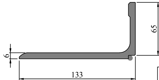
SEC. NO. IS00199 WEIGHT - 3.48 Kg/M
