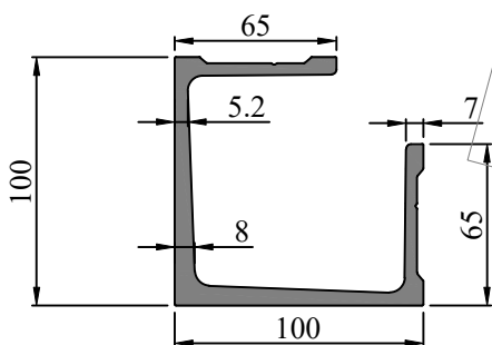
SEC. NO. FW0029 WEIGHT - 5.550 Kg/M
