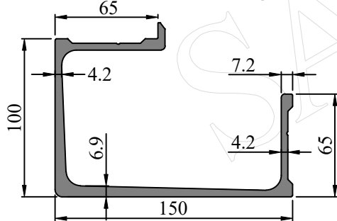
SEC. NO. FW0050 WEIGHT - 4.151 Kg/M
