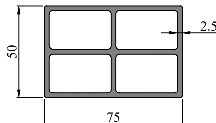
SEC. NO. FW0020 WEIGHT - 2.414 Kg/M
