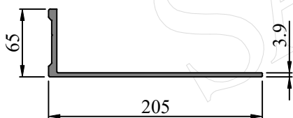
SEC. NO. FW0010 WEIGHT - 3.643 Kg/M
