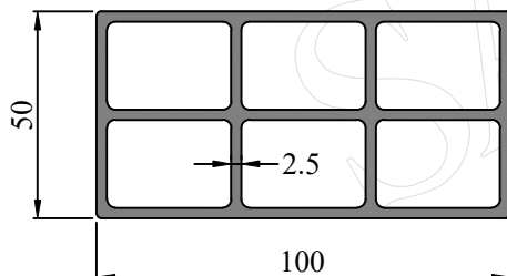
SEC. NO. IS00251 WEIGHT - 1.907 Kg/M
