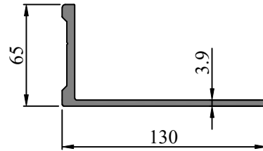
SEC. NO. FW0033 WEIGHT - 2.327 Kg/M
