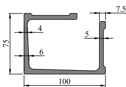
SEC. NO. FW0050 WEIGHT - 4.151 Kg/M
