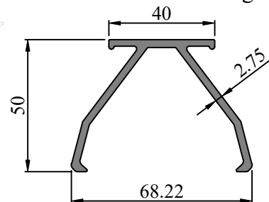
SEC. NO. FW0042 WEIGHT - 1.151 Kg/M
