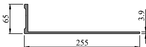
SEC. NO. FW0010 WEIGHT - 3.643 Kg/M
