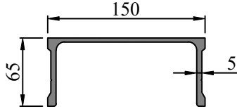
SEC. NO. FW0016 WEIGHT - 3.582 Kg/M
