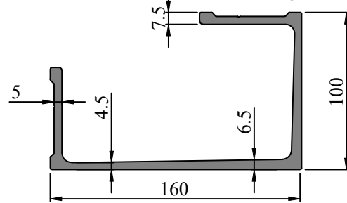
SEC. NO. FW0045 WEIGHT - 5.616 Kg/M
