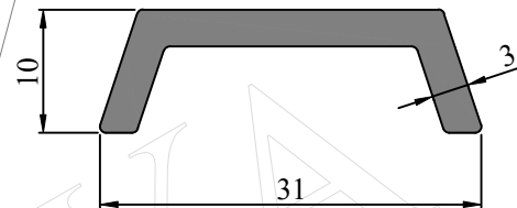
SEC. NO. IS00210 WEIGHT - 1.71 Kg/M
