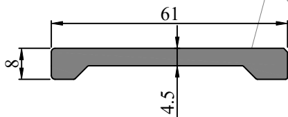
SEC. NO. FW0039 WEIGHT - 0.903 Kg/M
