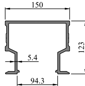
SEC. NO. FW0015 WEIGHT - 8.183 Kg/M
