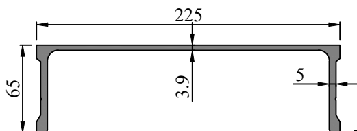
SEC. NO. FW0036 WEIGHT - 4.371 Kg/M
