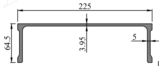
SEC. NO. FW0072 WEIGHT - 4.238 Kg/M
