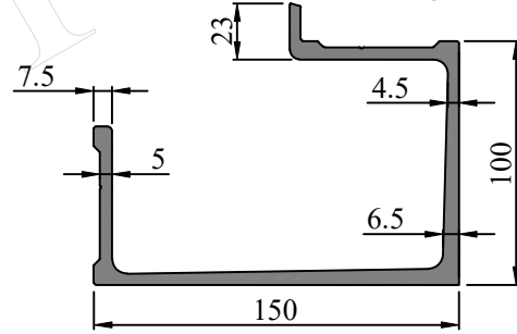
SEC. NO. FW0049 WEIGHT - 5.729 Kg/M
