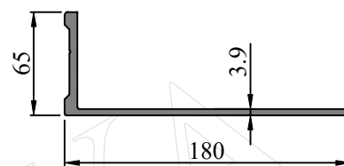
SEC. NO. FW0031 WEIGHT - 2.853 Kg/M
