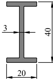
SEC. NO. IS00139 WEIGHT - 1.50 Kg/M
