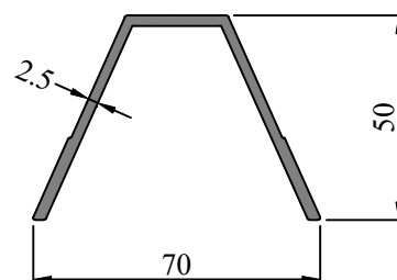
SEC. NO. IS00254 WEIGHT - 0.936 Kg/M
