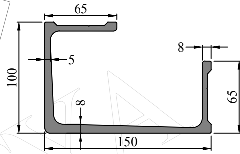
SEC. NO. FW0030 WEIGHT - 7.040 Kg/M
