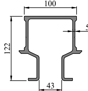
SEC. NO. FW0057 WEIGHT - 5.450 Kg/M
