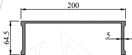
SEC. NO. FW0071 WEIGHT - 3.975 Kg/M
