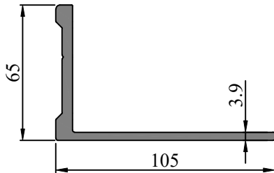
SEC. NO. FW0032 WEIGHT - 2.064 Kg/M
