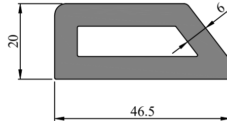
SEC. NO. IS00140 WEIGHT - 1.85 Kg/M
