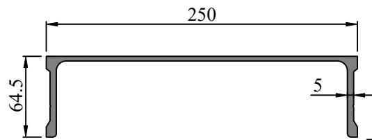
SEC. NO. FW0073 WEIGHT - 4.505 Kg/M
