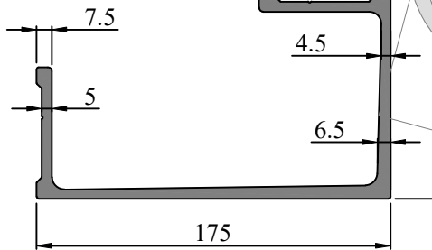
SEC. NO. FW0048 WEIGHT - 5.357 Kg/M
