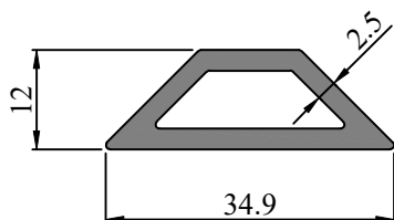
SEC. NO. FW0069 WEIGHT - 0.463 Kg/M
