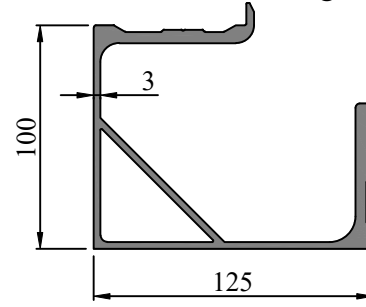
SEC. NO. FW0054 WEIGHT - 4.752 Kg/M
