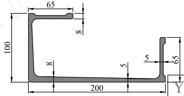
SEC. NO. FW0051 WEIGHT - 4.489 Kg/M
