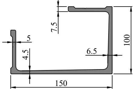
SEC. NO. FW0046 WEIGHT - 5.839 Kg/M
