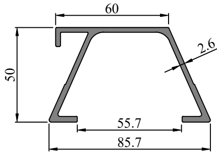
SEC. NO. FW0058 WEIGHT - 1.449Kg/M
