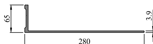
SEC. NO. FW0011 WEIGHT - 3.906 Kg/M
