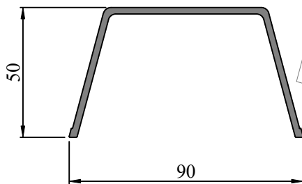
SEC. NO. IS00249 WEIGHT - 3.227 Kg/M
