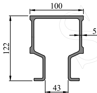
SEC. NO. FW0056 WEIGHT - 5.191 Kg/M
