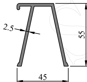
SEC. NO. IS0060 WEIGHT - 0.970 Kg/M
