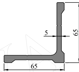
SEC. NO. FW0022 WEIGHT - 1.942 Kg/M
