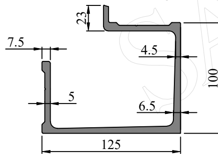
SEC. NO. FW0053 WEIGHT - 4.558 Kg/M
