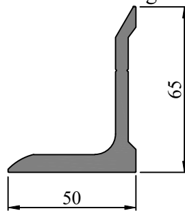
SEC. NO. IS00241 WEIGHT - 1.098 Kg/M
