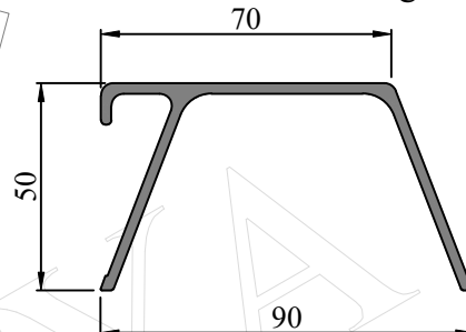
SEC. NO. IS00242 WEIGHT - 1.262 Kg/M
