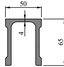
SEC. NO. IS00190 WEIGHT - 2.56 Kg/M
