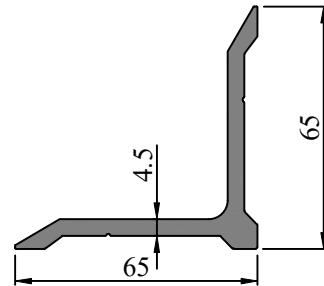
SEC. NO. FW0038 WEIGHT - 1.543Kg/M
