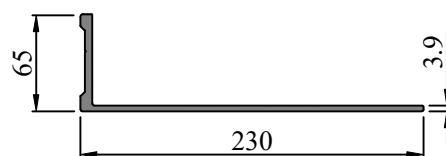
SEC. NO. FW0009 WEIGHT - 3.380 Kg/M
