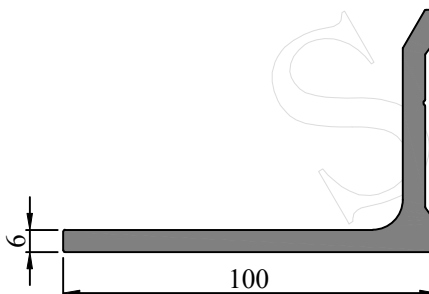
SEC. NO. FW0041 WEIGHT - 2.640 Kg/M
