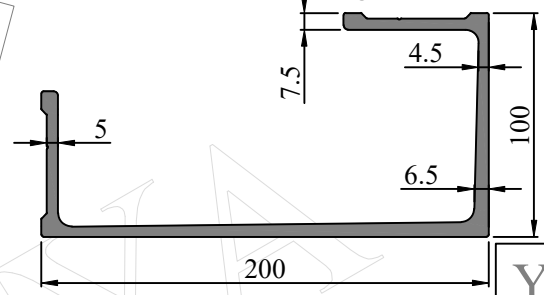
SEC. NO. FW0047 WEIGHT - 6.211 Kg/M
