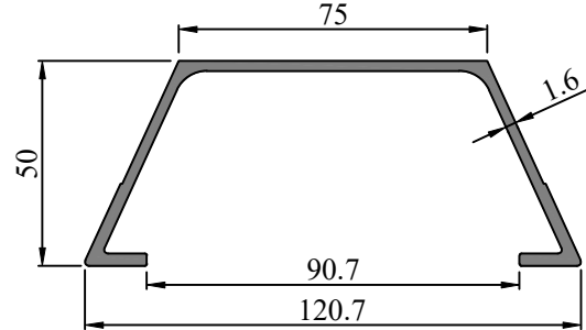
SEC. NO. FW0059 WEIGHT - 1.540 Kg/M
