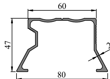
SEC. NO. FW0070 WEIGHT - 0.973 Kg/M
