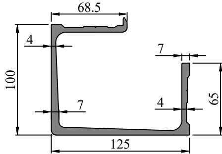
SEC. NO. FW0025 WEIGHT - 5.222 Kg/M
