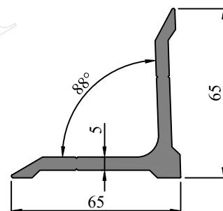
SEC. NO. IS00210 WEIGHT - 1.71 Kg/M
