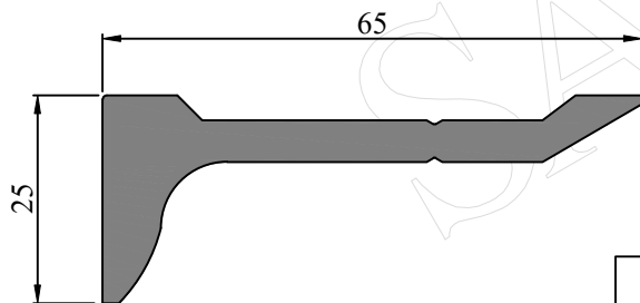
SEC. NO. IS00211 WEIGHT - 1.71 Kg/M
