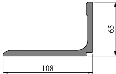
SEC. NO. IS00200 WEIGHT - 2.50 Kg/M
