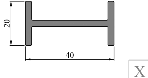
SEC. NO. FW0079 WEIGHT - 0.561 Kg/M
