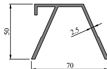
SEC. NO. IS00213 WEIGHT - 1.115 Kg/M
