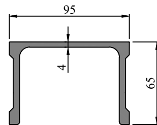
SEC. NO. IS00194 WEIGHT - 3.00 Kg/M
