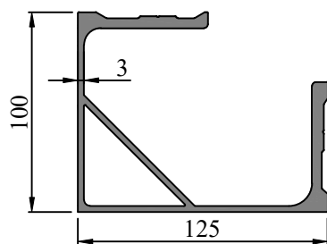
SEC. NO. FW0053 WEIGHT - 4.558 Kg/M
