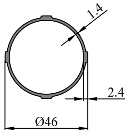
SEC. NO. IS00156 WEIGHT - 0.570 Kg/M
