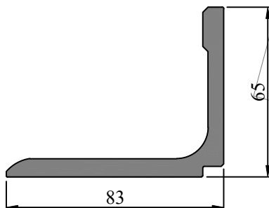
SEC. NO. IS00200 WEIGHT - 2.50 Kg/M
