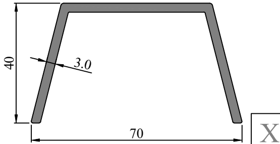
SEC. NO. FW0078 WEIGHT - 1.028 Kg/M
