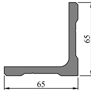
SEC. NO. IS00242 WEIGHT - 1.262 Kg/M
