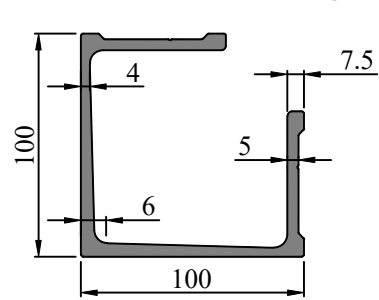
SEC. NO. FW0051 WEIGHT - 4.489 Kg/M
