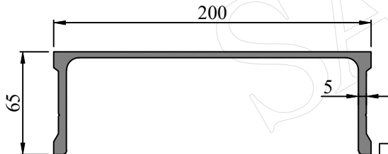
SEC. NO. FW0017 WEIGHT - 4.108 Kg/M
