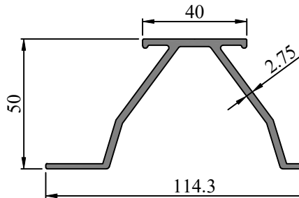
SEC. NO. FW0043 WEIGHT - 1.356 Kg/M
