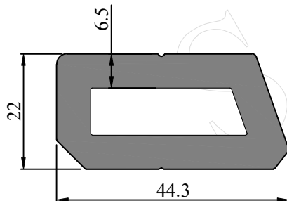
SEC. NO. FW0067 WEIGHT - 1.728 Kg/M
