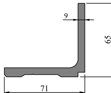
SEC. NO. IS00136R1 WEIGHT - 2.25 Kg/M
