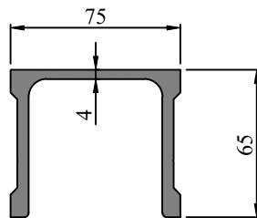
SEC. NO. IS00191 WEIGHT - 2.80 Kg/M
