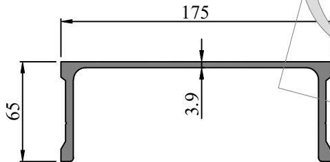
SEC. NO. FW0035 WEIGHT - 3.845 Kg/M
