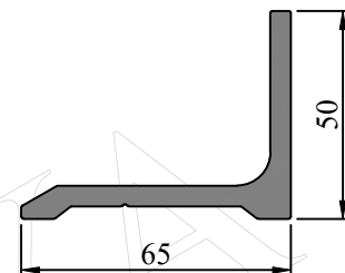
SEC. NO. FW0040 WEIGHT - 1.583 Kg/M
