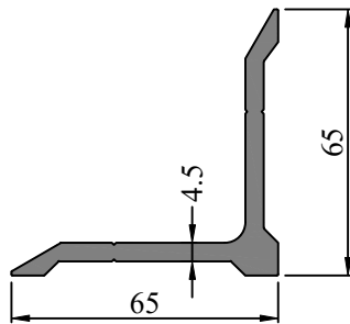
SEC. NO. FW0039 WEIGHT - 0.903 Kg/M
