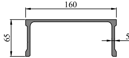
SEC. NO. FW0060 WEIGHT - 3.687 Kg/M
