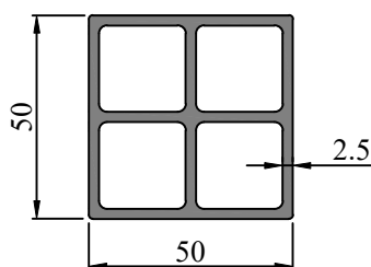
SEC. NO. IS00251 WEIGHT - 1.907 Kg/M
