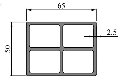
SEC. NO. IS00250 WEIGHT - 2.223 Kg/M
