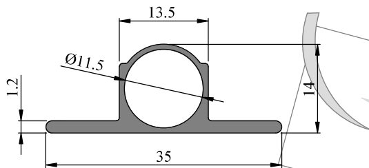
Profile Code - 341015 Weight KG /M - 0.241
