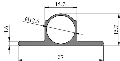
Profile Code - 341014 Weight KG /M - 0.186
