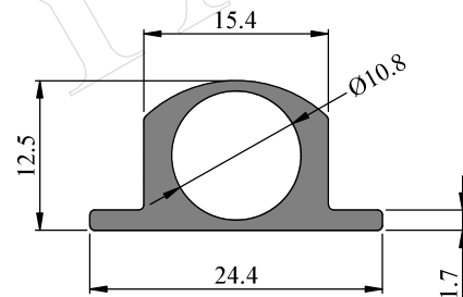
Profile Code - 341018 Weight./Mtr. (KG)- 0.273
