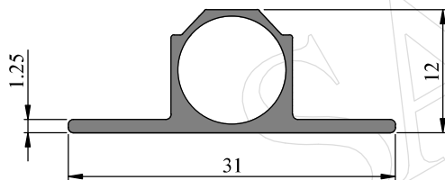
Profile Code - 332024 Weight KG /M - 1.65
