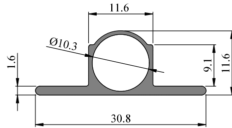
Profile Code - 341014 Weight KG /M - 0.186
