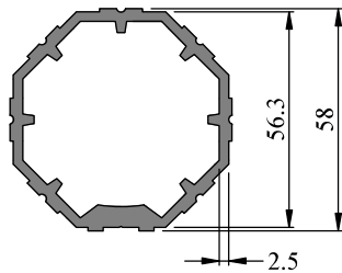
Profile Code - 332024 Weight KG /M - 1.65
