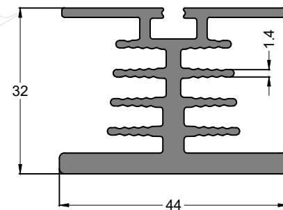
SEC. NO. IS00308 WEIGHT - 3.998 Kg/M
