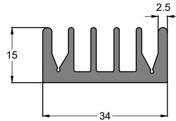
SEC. NO. IS0026
