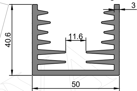
SEC. NO. IS00283 WEIGHT - 0.287 Kg/M
