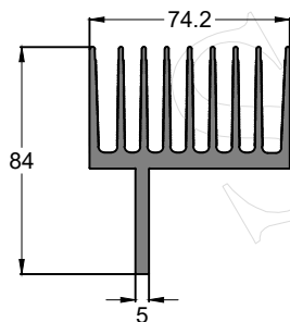
SEC.NO. IS00118 WEIGHT - 4.00 Kg/M
