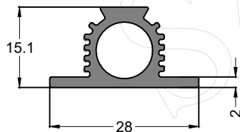
SEC. NO. IS00307 WEIGHT - 4.154 Kg/M
