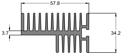
SEC. NO. IS0022
