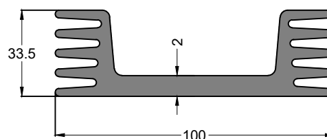
SEC. NO. IS00308 WEIGHT - 3.998 Kg/M
