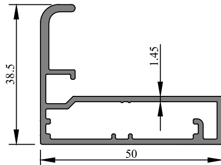
Profile Code - 366674 Weight (KG)/M - 0.721
