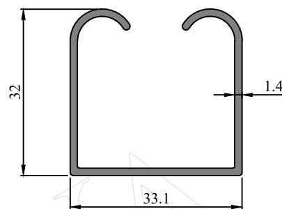
Profile Code - 366101 Weight (KG)/M - 0.420
