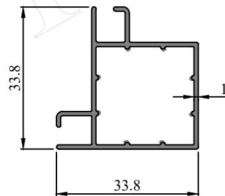
Profile Code - 366085 Weight (KG)/M - 0.377
