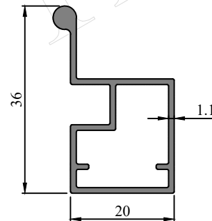
Profile Code - 366643 Weight (KG)/M - 0.347
