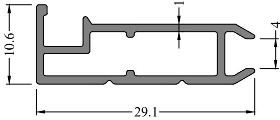
Profile Code - 366149 Weight KG /M - 0.212
