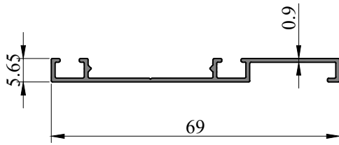
Profile Code - 366078 Weight (KG)/M - 0.251
