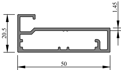
Profile Code - 366642 Weight (KG)/M - 0.272
