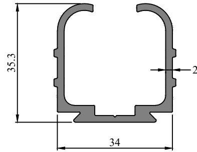
Profile Code - 452011 Weight (KG)/M - 0.695
