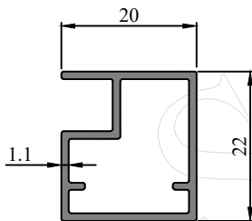
Profile Code - 366104 Weight (KG)/M - 1.165
