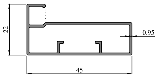
Profile Code - 366086 Weight (KG)/M - 0.368
