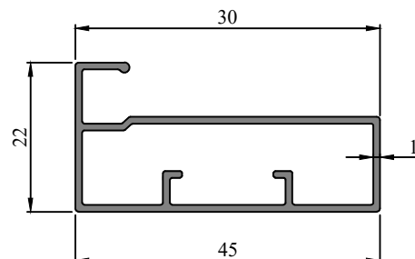
Profile Code - 366087 Weight (KG)/M - 0.386
