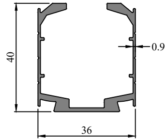
Profile Code - 366102 Weight (KG)/M - 0.604
