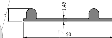
Profile Code - 452014 Weight (KG)/M - 0.343
