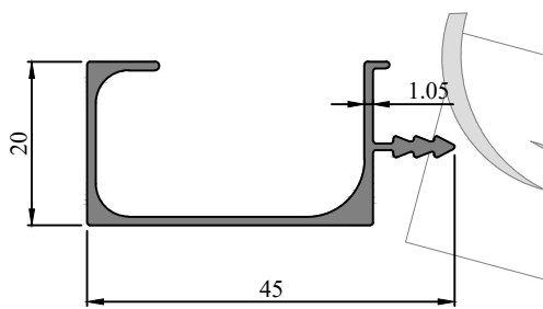
Profile Code - 366096 Weight (KG)/M - 0.321
