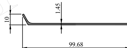
Profile Code - 452016 Weight (KG)/M - 0.413
