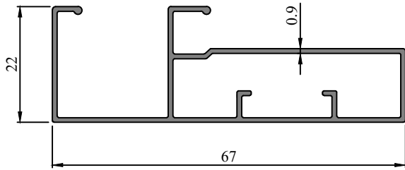
Profile Code - 366090 Weight (KG)/M - 0.470
