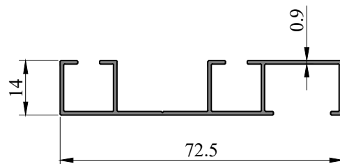
Profile Code - 366077 Weight KG /M - 0.380
