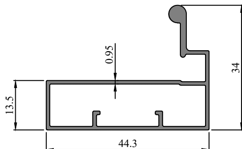
Profile Code - 366110 Weight (KG)/M - 0.452
