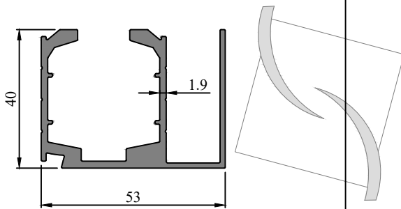
Profile Code - 366104 Weight (KG)/M - 1.165
