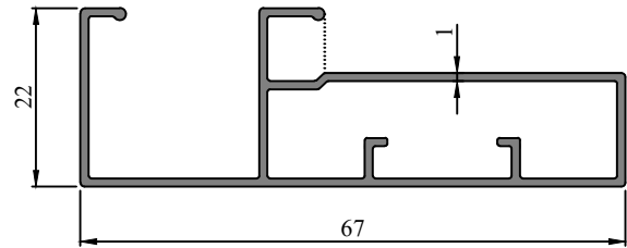
Profile Code - 366091 Weight (KG)/M - 0.516
