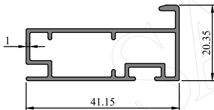
Profile Code - 366084 Weight (KG)/M - 0.381
