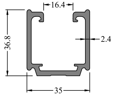
Profile Code - 366139 Weight KG /M - 0.822
