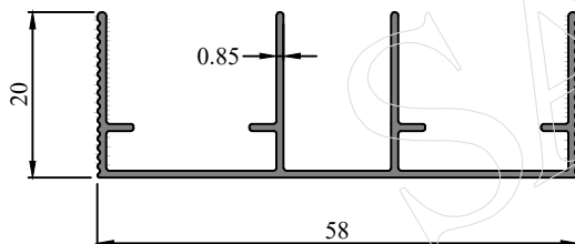
Profile Code - 452015 Weight (KG)/M - 0.346
