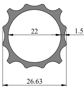
Profile Code - 335011 Weight(KG)/M - 0.464
