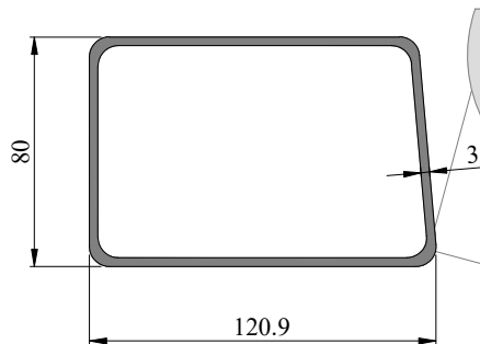
Profile Code - 353041 Weight(KG)/M - 3.115
