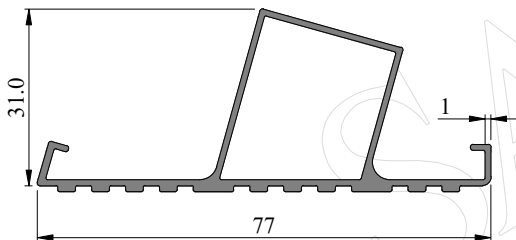
Profile Code - 352013 Weight(KG)/M - 0.587
