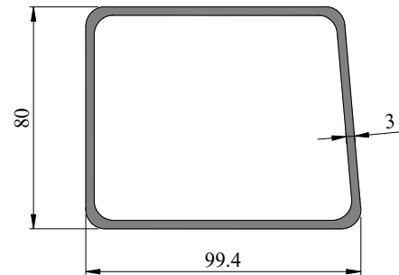
Profile Code - 353040 Weight(KG)/M - 2.765
