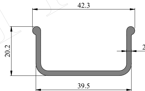
Profile Code - 353036 Weight(KG)/M - 0.407
