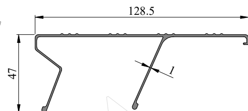
Profile Code - 353042 Weight(KG)/M - 0.778
