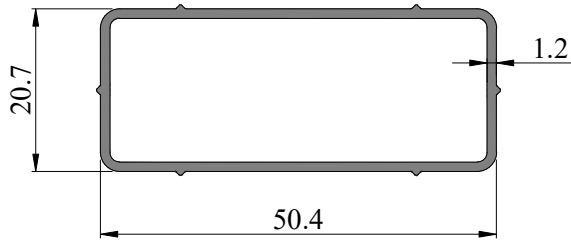
Profile Code - 353033 Weight KG /M - 0.439
