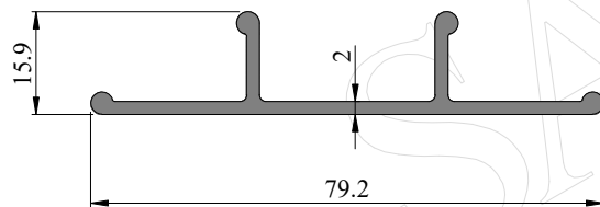
Profile Code - 353035 Weight(KG)/M - 0.615
