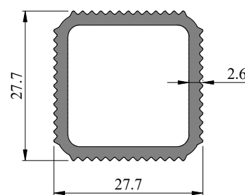
Profile Code - 353038 Weight(KG)/M - 0.575
