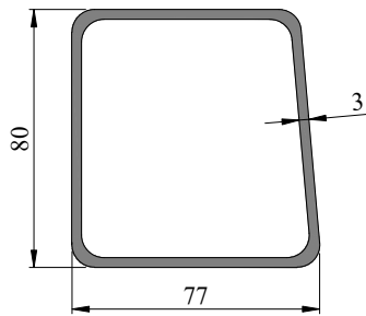
Profile Code - 353039 Weight(KG)/M - 2.402
