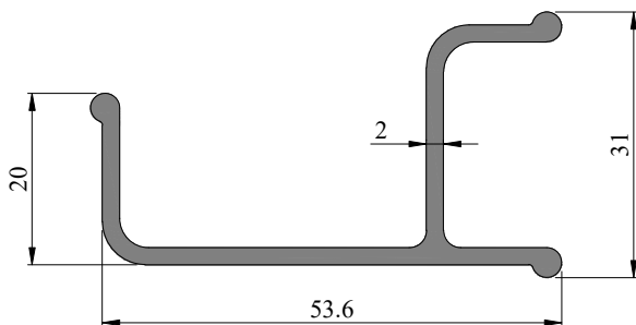
Profile Code - 353037 Weight(KG)/M - 0.617
