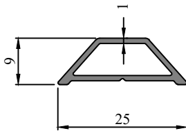
Profile Code - 431065 Weight (KG)/M - 0.145
