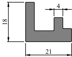
Profile Code - 431062 Weight (KG)/M - 0.500
