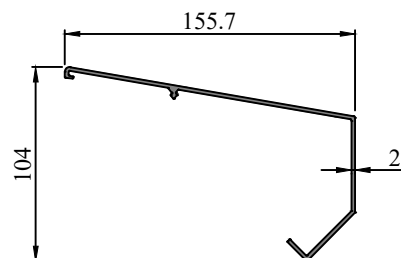
Profile Code - 431060 Weight (KG)/M - 1.456
