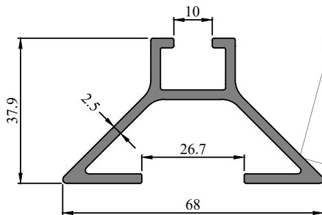
Profile Code - 431045 Weight (KG)/M - 1.052
