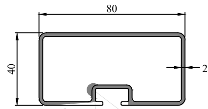
Profile Code - 431066 Weight (KG)/M - 1.362
