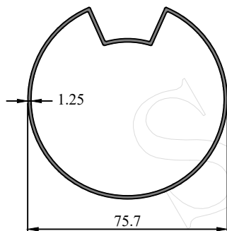
Profile Code - 431058 Weight (KG)/M - 0.845
