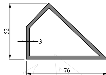
Profile Code - 403010 Weight/12' (KG) - 6.000-6.500
