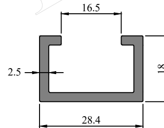
Profile Code - 431059 Weight (KG)/M - 0.448
