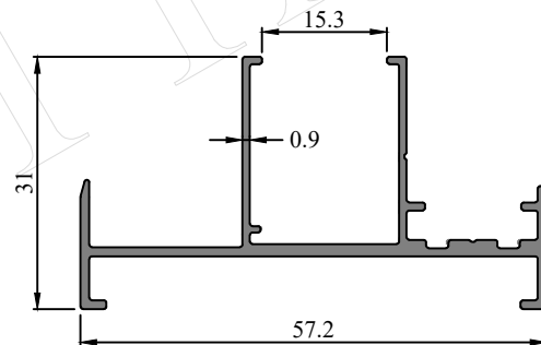
Profile Code - 431048 Weight (KG)/M - 0.445
