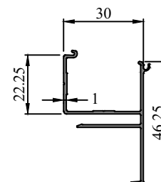
Profile Code - 431061 Weight (KG)/M - 1.466
