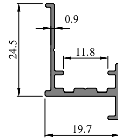
Profile Code - 431028 Weight (KG)/M - 0.198
