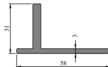
Profile Code - 431042 Weight (KG)/M - 0.847
