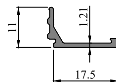
Profile Code - 431054 Weight (KG)/M - 0.106
