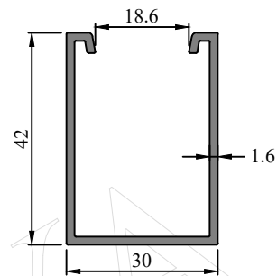
Profile Code - 431046 Weight (KG)/M - 0.529
