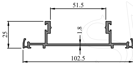
Profile Code - 431039 Weight (KG)/M - 0.924
