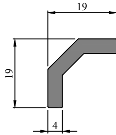
Profile Code - 431035 Weight (KG)/M - 0.321
