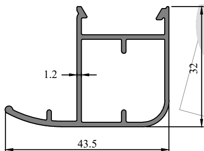
Profile Code - 431057 Weight (KG)/M - 0.463
