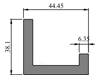
Profile Code - 431067 Weight (KG)/M - 1.442
