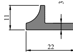
Profile Code - 431064 Weight (KG)/M - 0.254
