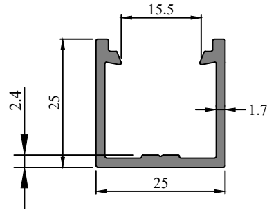
Profile Code - 431036 Weight (KG)/M - 0.389
