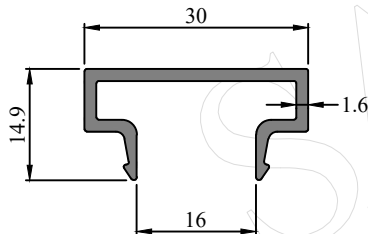
Profile Code - 431047 Weight (KG)/M - 0.279
