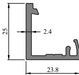
Profile Code - 431037 Weight (KG)/M - 0.341
