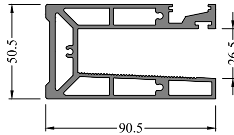
Profile Code - 366213 Weight KG /M - 3.160
