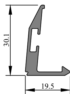
WEIGHT Kg/M : 0.322 SEC NO. 366202
