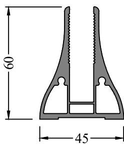
Profile Code - 366205 Weight KG /M - 1.513
