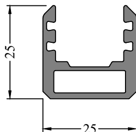
Profile Code - 366209 Weight KG /M - 0.512
