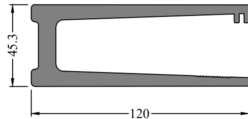
Profile Code - 366204 Weight KG /M - 5.268
