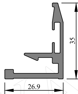
SEC NO. 366201 WEIGHT Kg/M : 0.513
