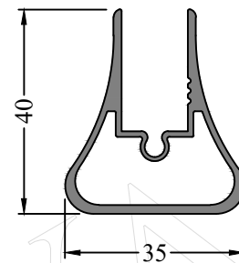
Profile Code - 366206 Weight KG /M - 0.616
