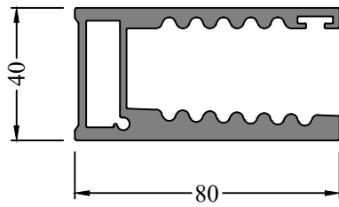
Profile Code - 366203 Weight KG /M - 2.747
