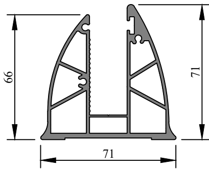
Profile Code - 366211 Weight KG /M - 2.309
