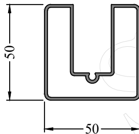
Profile Code - 366207 Weight KG /M - 1.078
