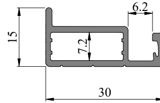
SEC. NO. SL0015 WEIGHT - 0.322 Kg/M
