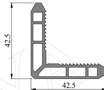
SEC. NO. SL0013 WEIGHT - 0.647 Kg/M
