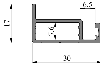
SEC. NO. SL0023 WEIGHT - 0.382 Kg/M
