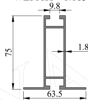
SEC. NO. 452029 WEIGHT - 1.183 Kg/M
