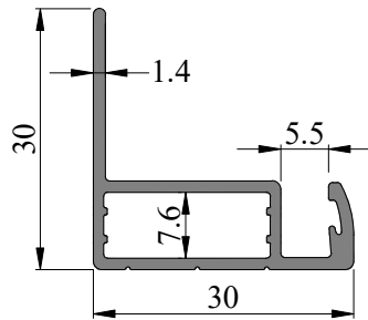
SEC. NO. SL0004 WEIGHT - 0.352 Kg/M
