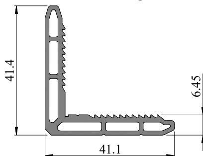
SEC. NO. SL0027 WEIGHT - 0.714Kg/M
