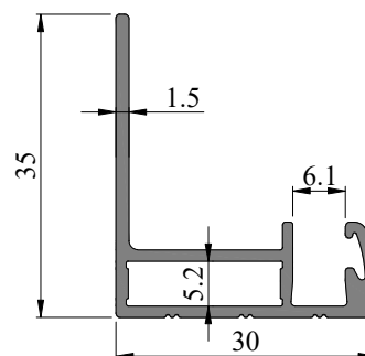
SEC. NO. SL0028 WEIGHT - 0.390 Kg/M
