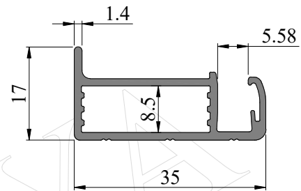
SEC. NO. IS00173 WEIGHT - 0.300 Kg/M
