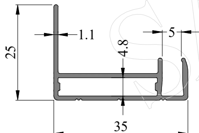
SEC. NO. IS0091 WEIGHT - 0.320 Kg/M
