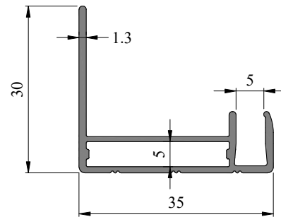
SEC. NO. IS00248 WEIGHT - 0.362 Kg/M
