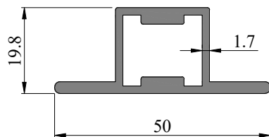
SEC. NO. IS00232 WEIGHT - 1.02 Kg/M
