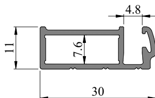
SEC. NO. SL0024 WEIGHT - 0.284 Kg/M
