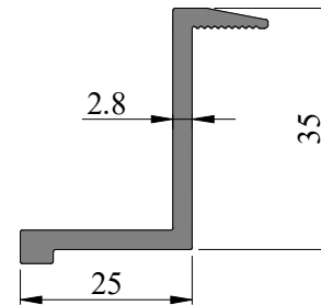
SEC. NO. 452029 WEIGHT - 1.183 Kg/M
