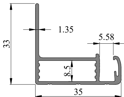
SEC. NO. SL0009 WEIGHT - 0.394 Kg/M
