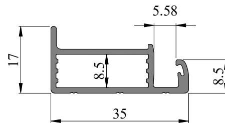
SEC. NO. SL0010 WEIGHT - 0.321 Kg/M
