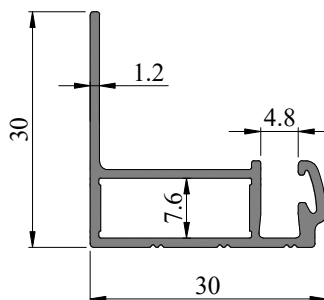
SEC. NO. SL0018 WEIGHT - 0.329 Kg/M
