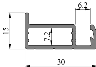
SEC. NO. SL0022 WEIGHT - 0.317 Kg/M
