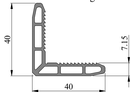
SEC. NO. SL0013 WEIGHT - 0.647 Kg/M
