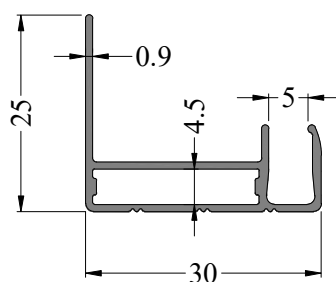
SEC. NO. IS00111 WEIGHT - 0.240 Kg/M
