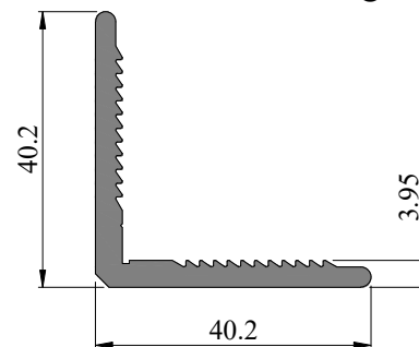
SEC. NO. 411017 WEIGHT - 0.712 Kg/M
