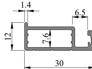
SEC. NO. SL0005 WEIGHT - 0.275 Kg/M
