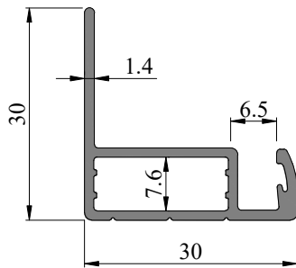
SEC. NO. SL0022 WEIGHT - 0.317 Kg/M
