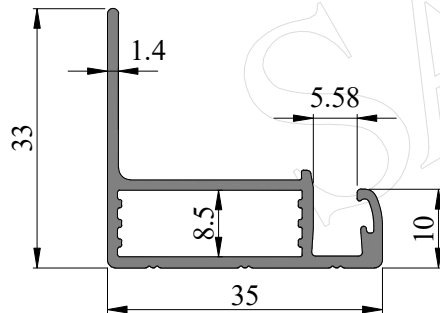
SEC. NO. SL0009 WEIGHT - 0.394 Kg/M
