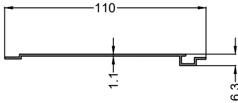
Profile Code - IS00179 Weight KG /M - 0.363
