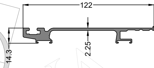
Profile Code - IS00148 Weight KG /M - 1.30
