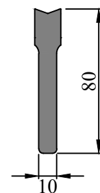
SEC. NO. IS00151 WEIGHT - 2.40 Kg/M
