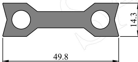
SEC. NO. IS00121 WEIGHT - 1.550 Kg/M
