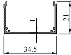
SEC. NO. IS0088 WEIGHT - 0.600 Kg/M
