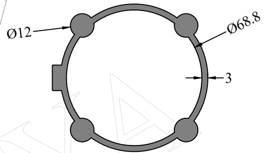
SEC.NO. IS0004 WEIGHT - 2.80 Kg/M
