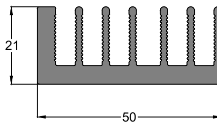
SEC. NO. IS00202 WEIGHT - 1.33 Kg/M
