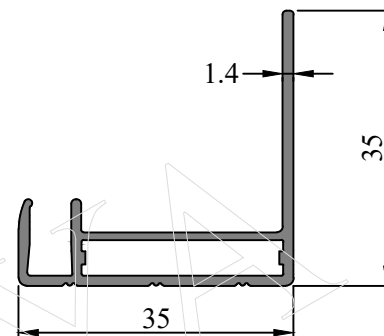
SEC. NO. IS00172 WEIGHT - 0.280 Kg/M
