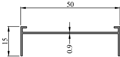
SEC. NO. IS00218 WEIGHT - 8.418 Kg/M
