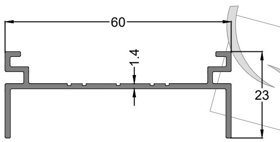
Profile Code - IS00181 Weight KG /M - 0.432
