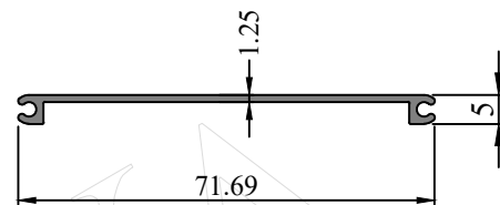
SEC. NO. IS0089 WEIGHT - 0.345 Kg/M
