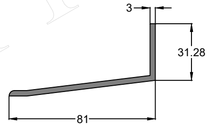
Profile Code - IS00175 Weight KG /M - 0.885
