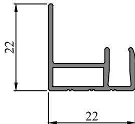
SEC. NO. IS0090 WEIGHT - 0.230 Kg/M
