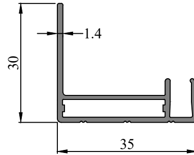
SEC. NO. IS00143 WEIGHT - 0.365 Kg/M
