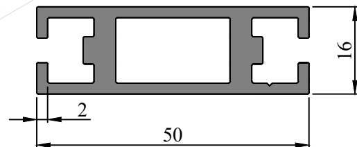
SEC. NO. IS0054 WEIGHT - 0.930 Kg/M
