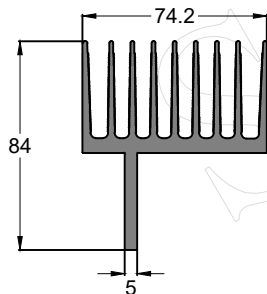
SEC.NO. IS00118 WEIGHT - 4.00 Kg/M
