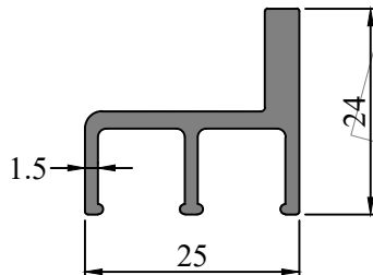
SEC. NO. IS0012 WEIGHT - 0.395 Kg/M
