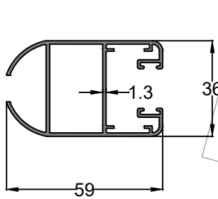
Profile Code - IS0077 Weight KG /M - 0.850
