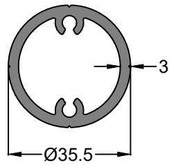
Profile Code - IS00132 Weight KG /M - 0.150
