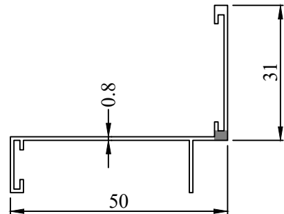
SEC. NO. IS00109 WEIGHT - 0.600 Kg/M
