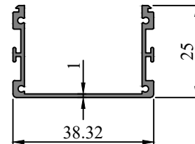
SEC. NO. IS00152 WEIGHT - 0.330 Kg/M
