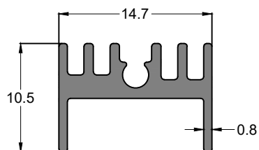
SEC. NO. IS0046
