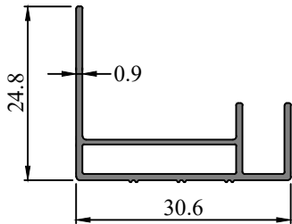
SEC. NO. IS00233 WEIGHT - 0.510 Kg/M
