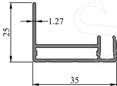
SEC. NO. IS0092 WEIGHT - 0.350 Kg/M
