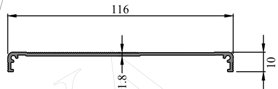
SEC. NO. IS00131R2 WEIGHT - 0.570 Kg/M
