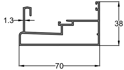
Profile Code - IS0076 Weight KG /M - 0.866
