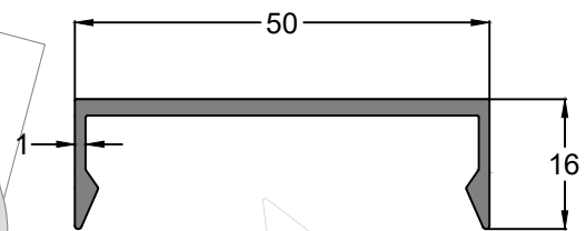
Profile Code - IS0099 Weight KG /M - 0.390
