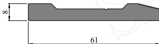
SEC. NO. IS0019 WEIGHT - 1.10 Kg/M
