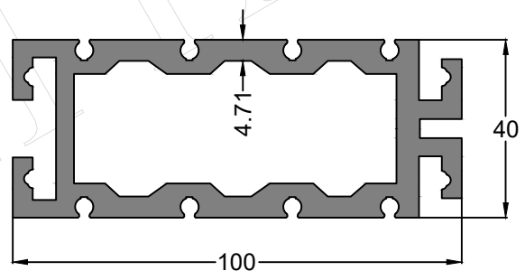
Profile Code - IS0099 Weight KG /M - 0.390
