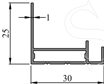
SEC. NO. IS00150 WEIGHT - 0.240 Kg/M
