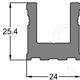
Profile Code - IS00207 Weight KG /M - 1.10
