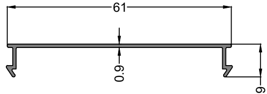
Profile Code - IS00180 Weight KG /M - 0.196
