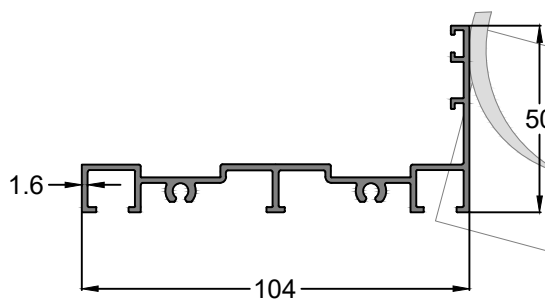
Profile Code - IS0085 Weight KG /M - 1.10
