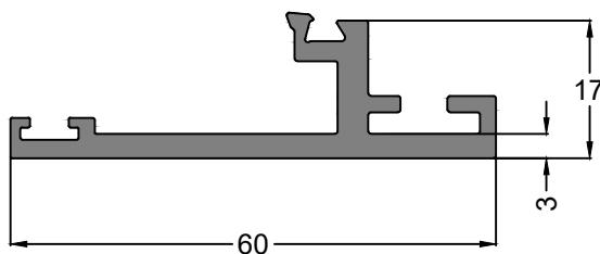
Profile Code - IS00105 Weight KG /M - 0.760
