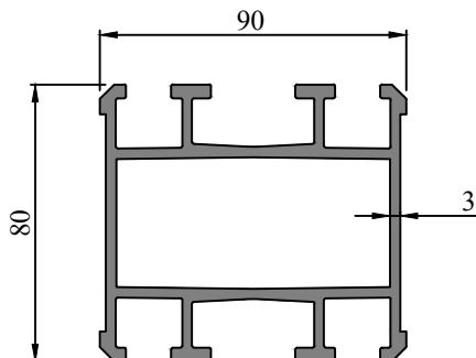
SEC. NO. IS00204 WEIGHT - 3.75 Kg/M
