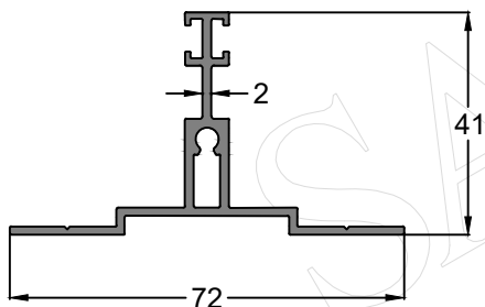
Profile Code - IS0079 Weight KG /M - 1.10
