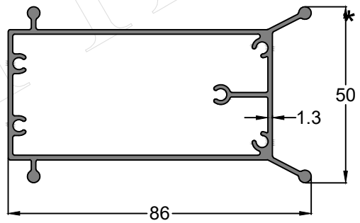
Profile Code - IS00184 Weight KG /M - 1.15
