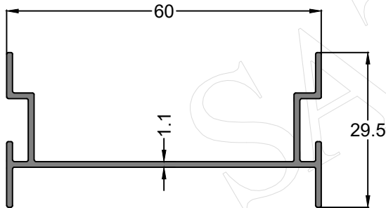
Profile Code - IS00183 Weight KG /M - 0.393
