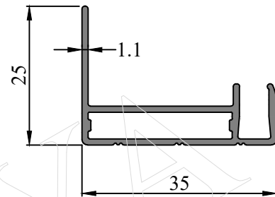
SEC. NO. IS0091 WEIGHT - 0.320 Kg/M
