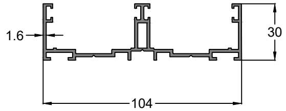
Profile Code - IS0084 Weight KG /M - 1.10
