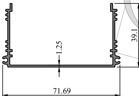
SEC. NO. IS0088 WEIGHT - 0.600 Kg/M
