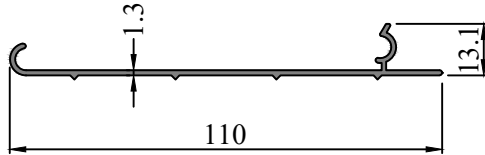
SEC. NO. IS0047 WEIGHT - 0.470 Kg/M
