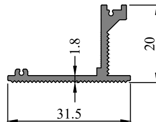
SEC.NO. IS0096 WEIGHT - 0.280 Kg/M
