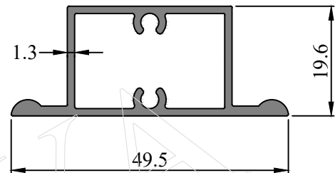
SEC. NO. IS0051 WEIGHT - 0.490 Kg/M
