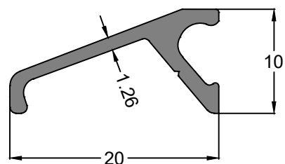
Profile Code - IS00108 Weight KG /M - 1.30
