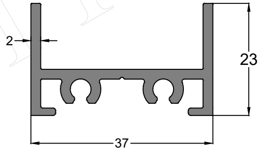
Profile Code - IS0080 Weight KG /M - 0.566
