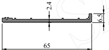
SEC.NO. IS0095 WEIGHT - 0.430 Kg/M
