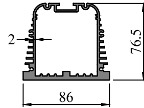
SEC. NO. IS0056 WEIGHT - 1.20 Kg/M
