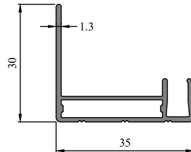
SEC. NO. IS0053 WEIGHT - 0.330 Kg/M
