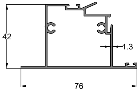
Profile Code - IS0075 Weight KG /M - 0.850
