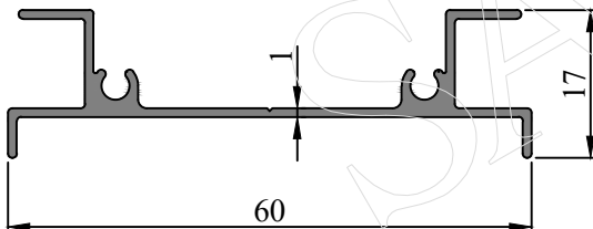
SEC. NO. IS0052 WEIGHT - 0.360 Kg/M
