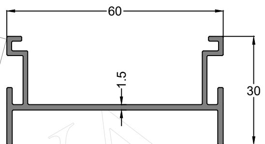
Profile Code - IS00182 Weight KG /M - 0.542
