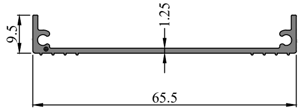
SEC. NO. IS00222 WEIGHT - 0.317 Kg/M
