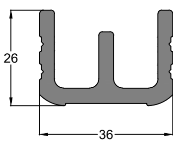
Profile Code - IS00205 Weight KG /M - 1.00
