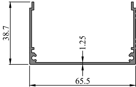
SEC. NO. IS00221 WEIGHT - 0.570 Kg/M
