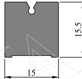
SEC. NO. IS00109 WEIGHT - 0.600 Kg/M
