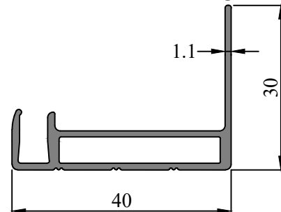
SEC. NO. IS0093 WEIGHT - 0.390 Kg/M
