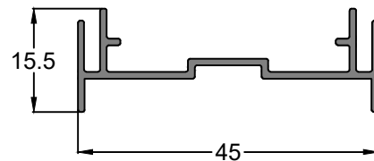
Profile Code - IS00178 Weight KG /M - 0.258
