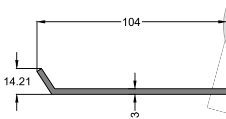
Profile Code - IS00132 Weight KG /M - 0.150
