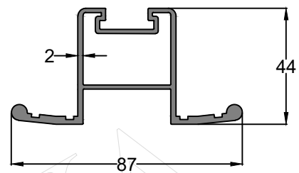
Profile Code - IS0078 Weight KG /M - 1.30
