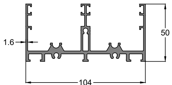
Profile Code - IS0082 Weight KG /M - 2.10
