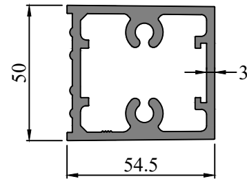
SEC. NO. IS0033 WEIGHT - 0.470 Kg/M
