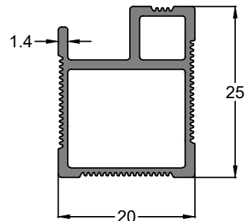
Profile Code - IS00186 Weight KG /M - 0.307
