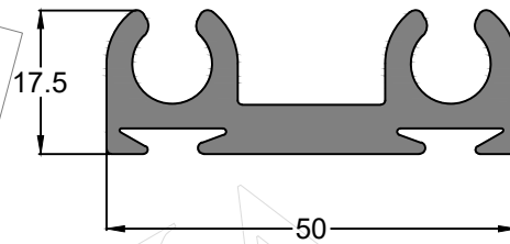
Profile Code - IS00206 Weight KG /M - 1.10
