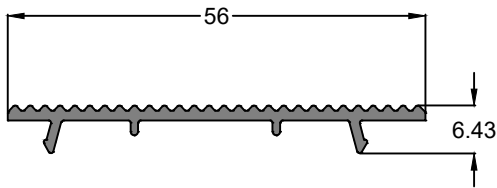
Profile Code - IS0083 Weight KG /M - 0.290
