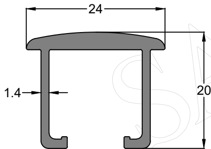
Profile Code - IS00149 Weight KG /M - 0.315
