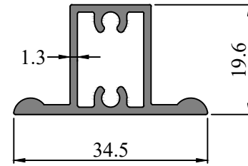
SEC. NO. IS0048 WEIGHT - 0.390 Kg/M
