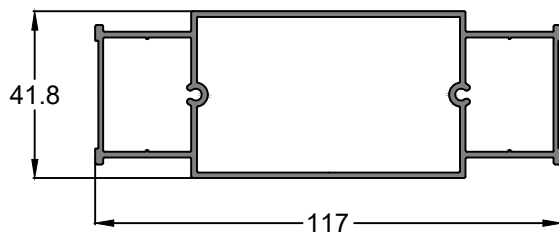
Profile Code - IS00177 Weight KG /M - 3.43
