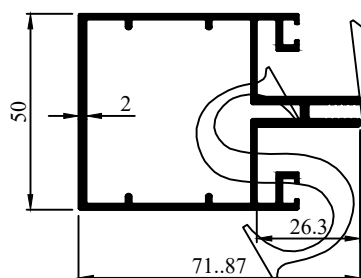
Profile Code - 272042 Weight KG /M - 1.335
