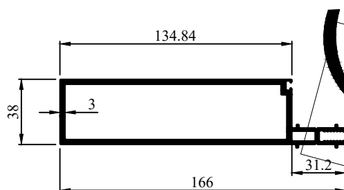
Profile Code - 273016 Weight KG /M - 3.119
