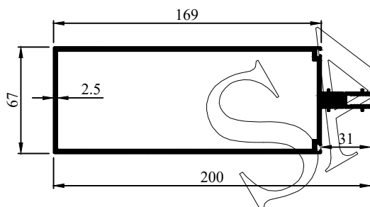
Profile Code - 272028 Weight KG /M - 3.766
