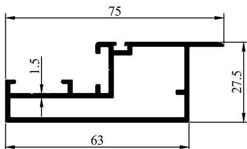
Profile Code - 541012 Weight KG /M - 0.868
