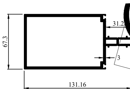
Profile Code - 272022 Weight KG /M - 3.00
