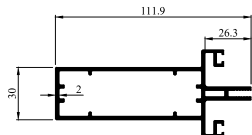
Profile Code - 272043 Weight KG /M - 2.422
