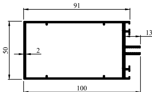
Profile Code - 271312 Weight KG /M - 1.528
