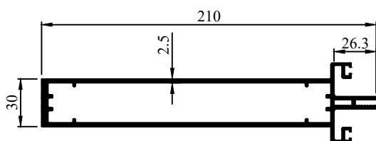
Profile Code - 272044 Weight KG /M - 3.600
