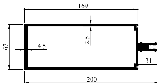
Profile Code - 272031 Weight KG /M - 4.101
