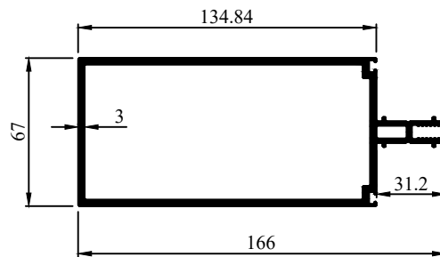
Profile Code - 272025 Weight KG /M - 3.602
