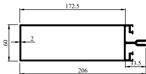
Profile Code - 272032 Weight KG /M - 3.272
