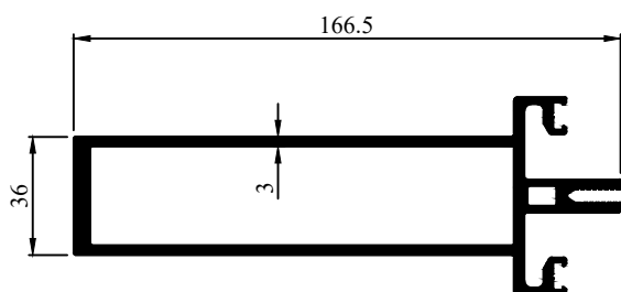
Profile Code - 272046 Weight KG /M - 3.878
