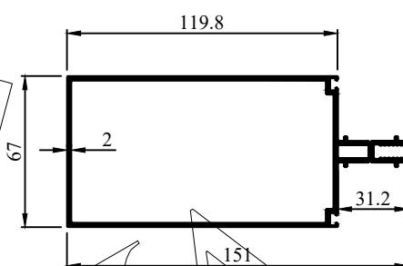
Profile Code - 272027 Weight KG /M - 2.561
