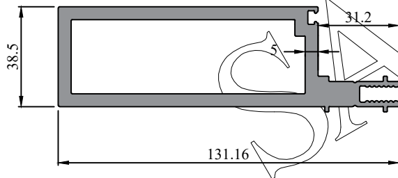
Profile Code - 273014 Weight KG /M - 4.10
