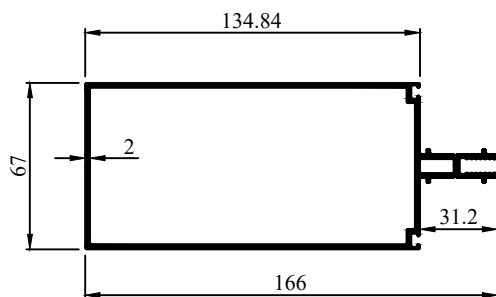
Profile Code - 272024 Weight KG /M - 2.566
