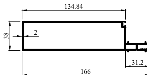
Profile Code - 273015 Weight KG /M - 2.240
