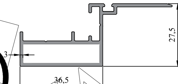
Profile Code - 542010 Weight KG /M - 0.830
