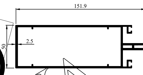
Profile Code - 272033 Weight KG /M - 2.562
