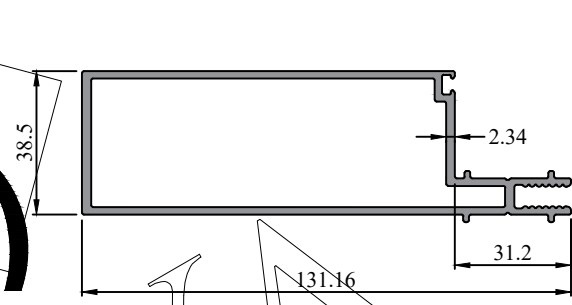
Profile Code - 273010 Weight KG /M - 1.90
