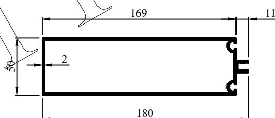
Profile Code - 272027 Weight KG /M - 2.561
