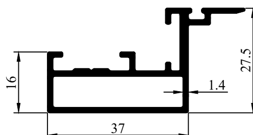
Profile Code - 541013 Weight KG /M - 0.614
