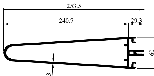
Profile Code - 272047 Weight KG /M - 5.447
