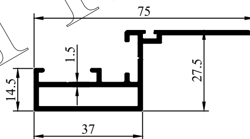
Profile Code - 541011 Weight KG /M - 0.683
