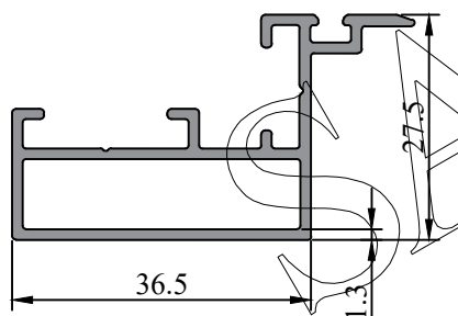
Profile Code - 541010 Weight KG /M - 0.520
