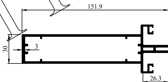
Profile Code - 272043 Weight KG /M - 2.422
