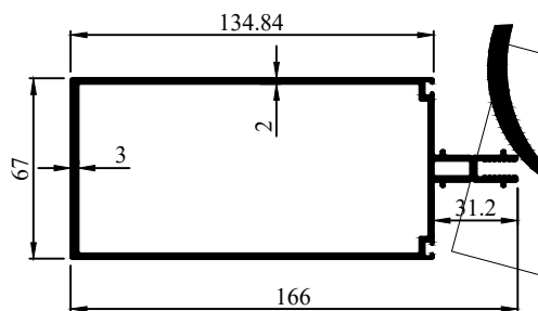
Profile Code - 272026 Weight KG /M - 2.736
