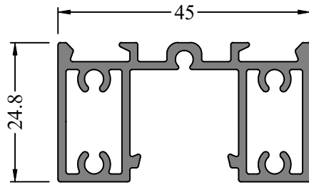
Profile Code - 366113 Weight KG /M - 0.789
