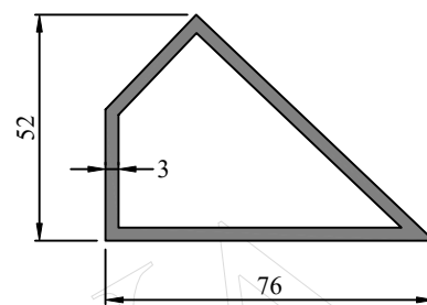
Profile Code - 403010 Weight/12' (KG) - 6.000-6.500
