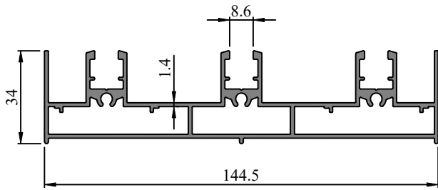
Profile Code - 366093 Weight KG /M - 2.207
