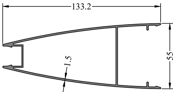
Profile Code - 366168 Weight KG /M - 1.477
