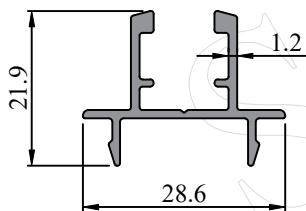
Profile Code - 363022 Weight KG /M - 0.262
