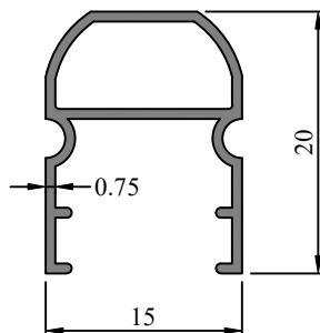
Profile Code - 431010 Weight/12' (KG) - 0.350-0.450
