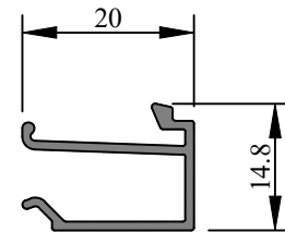
Profile Code - 366114 Weight KG /M - 0.328
