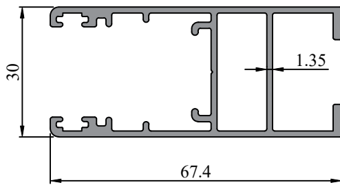
Profile Code - 363018 Weight KG /M - 0.932
