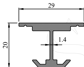
Profile Code - 431015 Weight (KG)/M - 0.355
