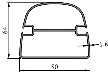
Profile Code - 431011 Weight (KG)/M - 1.668
