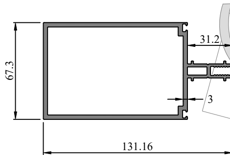
Profile Code - 272022 Weight KG /M - 3.00
