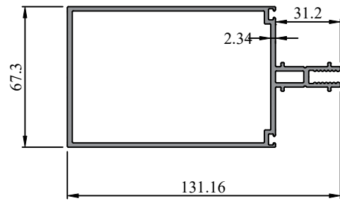
Profile Code - 272020 Weight KG /M - 2.30
