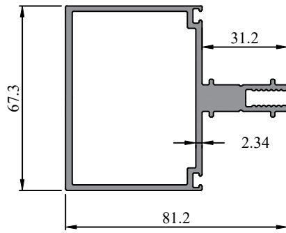
Profile Code - 272010 Weight KG /M - 1.80
