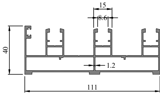
Profile Code - 366176 Weight (KG)/M - 1.757
