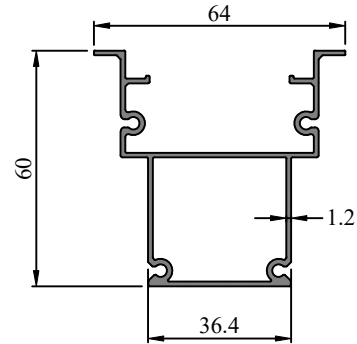
Profile Code - 431056 Weight (KG)/M - 0.884
