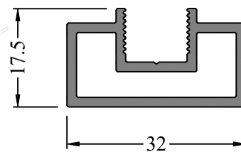
Profile Code - 366132 Weight KG /M - 0.479
