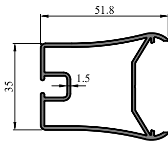
Profile Code - 431013 Weight (KG)/M - 0.791
