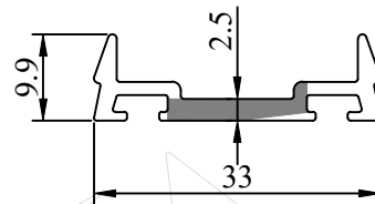
Profile Code - 366185 Weight KG /M - 0.286
