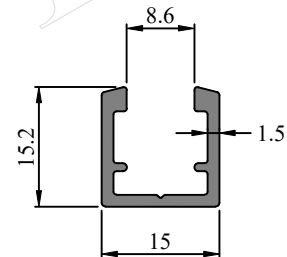
Profile Code - 366181 Weight (KG)/M - 0.202
