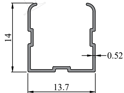
Profile Code - 404014 Weight (KG)/M - 0.062
