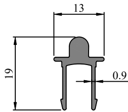
Profile Code - 366063 Weight KG /M - 0.121
