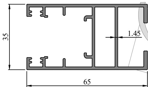
Profile Code - 363020 Weight KG /M - 1.035
