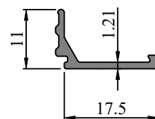
Profile Code - 431054 Weight (KG)/M - 0.106
