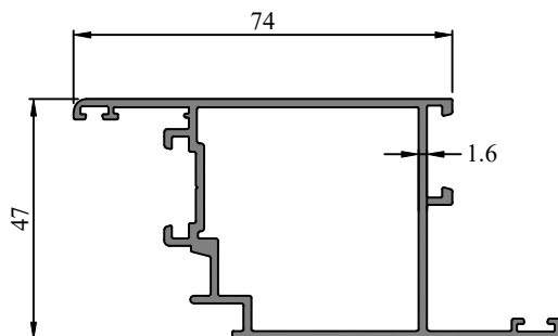
Profile Code - 366163 Weight (KG)/M - 0.932
