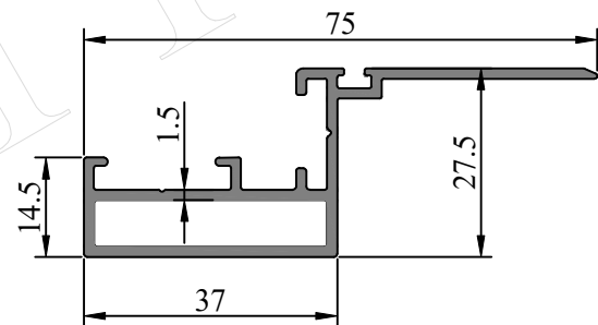
Profile Code - 541011 Weight KG /M - 0.683
