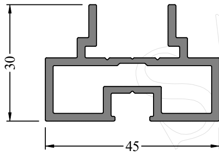
Profile Code - 366131 Weight KG /M - 0.859
