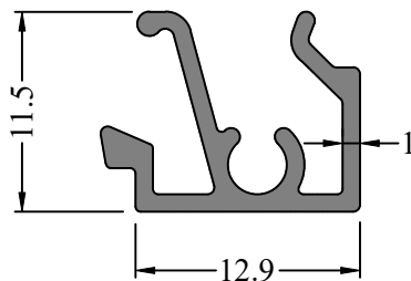
Profile Code - 366119 Weight KG /M - 0.139
