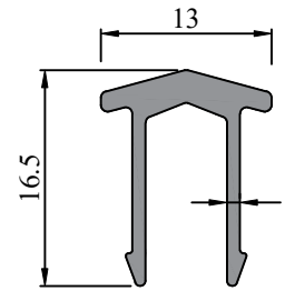
Profile Code - 363030 Weight KG /M - 0.151
