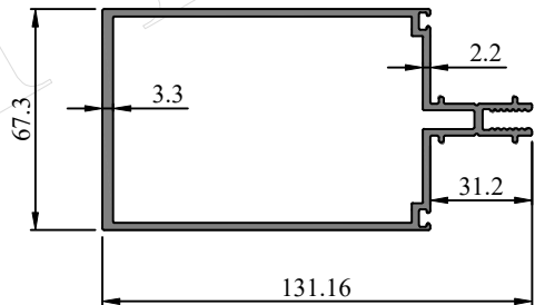
Profile Code - 272023 Weight KG /M - 2.51
