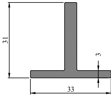
Profile Code - 431043 Weight (KG)/M - 0.644
