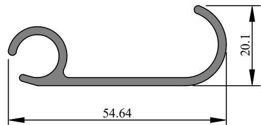
Profile Code - 3663001 Weight KG /M - 0.511
