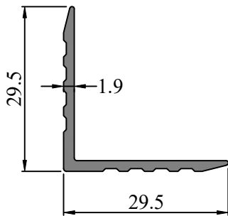
Profile Code - 421010 Weight KG /M - 0.250
