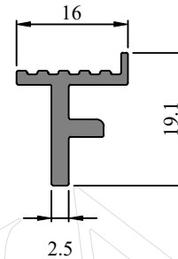
Profile Code - 431022 Weight (KG)/M - 0.214
