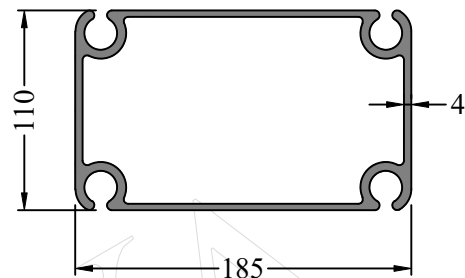
Profile Code - 3663004 Weight KG /M - 7.766
