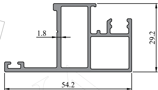
Profile code - 366046 Weight KG /M - 0.694
