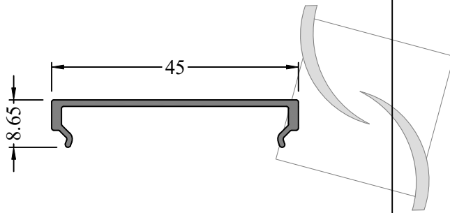
Profile Code - 366123 Weight KG /M - 0.209
