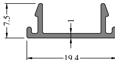
Profile Code - 366120 Weight KG /M - 0.099
