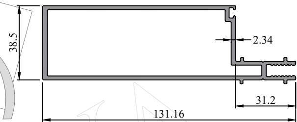
Profile Code - 273010 Weight KG /M - 1.90
