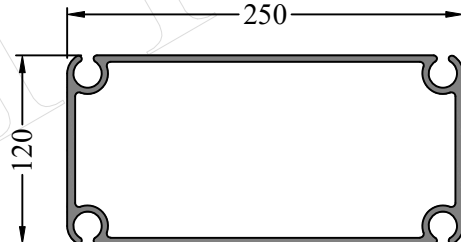
Profile Code - 3663004 Weight KG /M - 7.766
