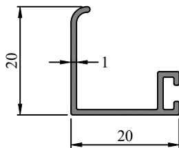
Profile Code - 366178 Weight (KG)/M - 0.144
