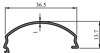
Profile Code - 431012 Weight (KG)/M - 1.291
