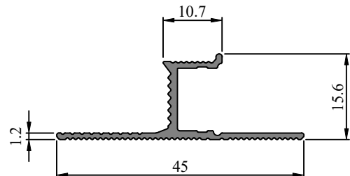
Profile Code - 431024 Weight (KG)/M - 0.327
