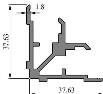
Profile Code - 431017 Weight (KG)/M - 0.787
