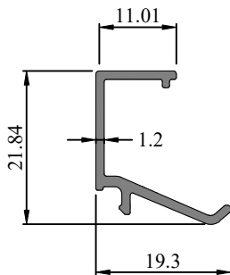
Profile Code - 366610 Weight (KG)/M - 0.650
