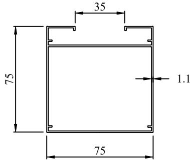
Profile Code - 431019 Weight (KG)/M - 1.052
