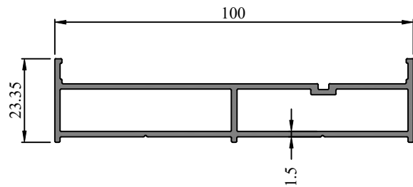
Profile Code - 366613 Weight (KG)/M - 1.054
