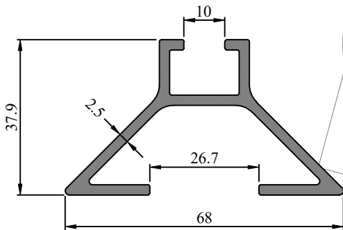
Profile Code - 431045 Weight (KG)/M - 1.052
