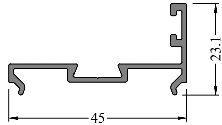
Profile Code - 366114 Weight KG /M - 0.328
