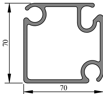
Profile Code - 3663001 Weight KG /M - 2.723
