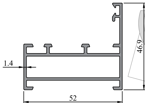
Profile Code - 366010 Weight KG /M - 0.789
