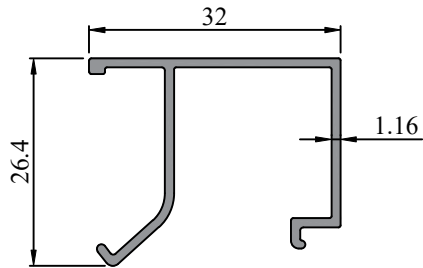
Profile Code - 245012 Weight KG /M - 0.289
