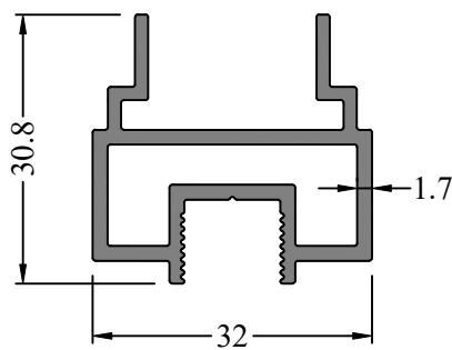
Profile Code - 366133 Weight KG /M - 0.611
