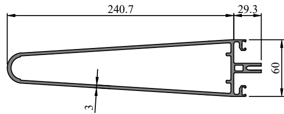
Profile Code - 272047 Weight KG /M - 5.447
