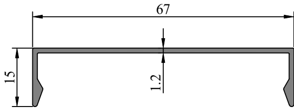
Profile Code - 366182 Weight KG /M - 0.331
