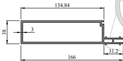
Profile Code - 273016 Weight KG /M - 3.119
