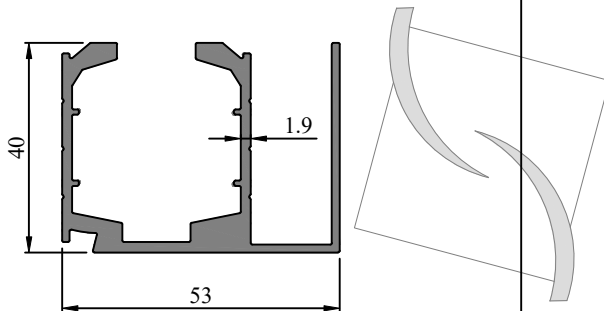
Profile Code - 366104 Weight (KG)/M - 1.165
