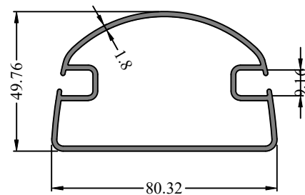
Profile Code - 431012 Weight (KG)/M - 1.291
