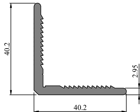
Profile Code - 411017 Weight KG /M - 0.712
