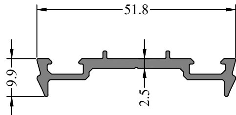
Profile Code - 366169 Weight KG /M - 0.424
