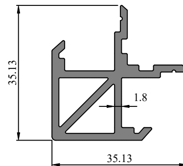
Profile Code - 431018 Weight (KG)/M - 0.721
