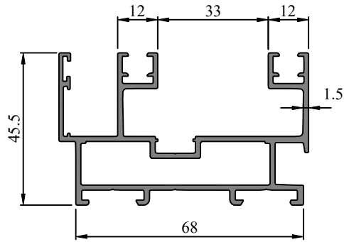
Profile Code - 366159 Weight (KG)/M - 1.377
