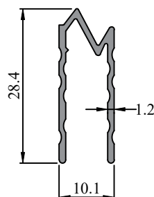
Profile Code - 422010 Weight KG /M - 0.180
