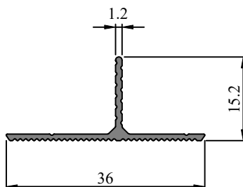
Profile Code - 431025 Weight (KG)/M - 0.146
