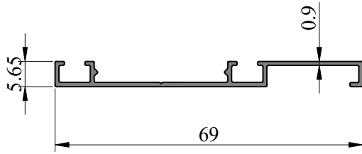
Profile Code - 366078 Weight KG /M - 0.251
