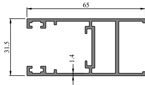
Profile Code - 366609 Weight (KG)/M - 0.622
