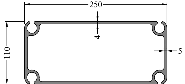
Profile Code - 3663006 Weight KG /M - 9.275
