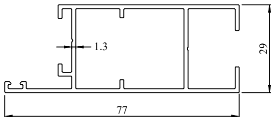
Profile Code - 366614 Weight (KG)/M - 0.790
