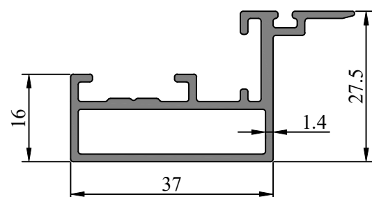
Profile Code - 541013 Weight KG /M - 0.614
