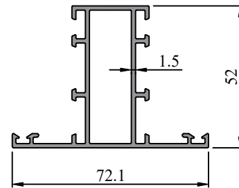
Profile code - 366030 Weight KG /M - 1.05
