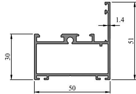
Profile Code - 366160 Weight (KG)/M - 0.859
