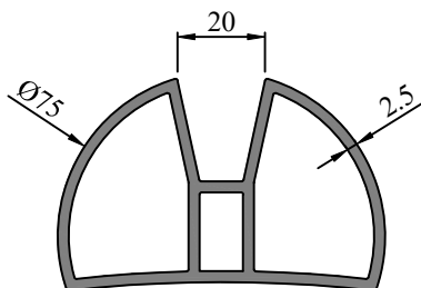
Profile Code - 431049 Weight (KG)/M - 1.887
