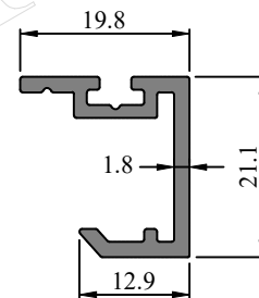
Profile Code - 431016 Weight (KG)/M - 0.280
