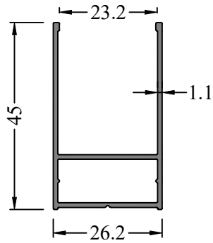
Profile Code - 366409 Weight KG /M - 0.415
