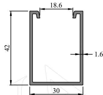
Profile Code - 431046 Weight (KG)/M - 0.529
