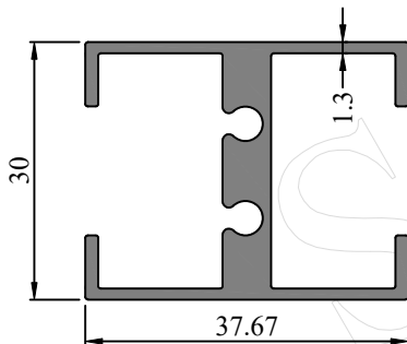
SEC. NO. 363023 WEIGHT - 0.704 Kg/M
