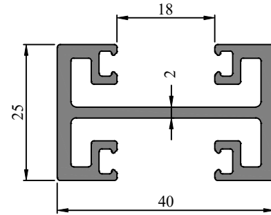
Profile Code - 366187 Weight (KG)/M - 0.854
