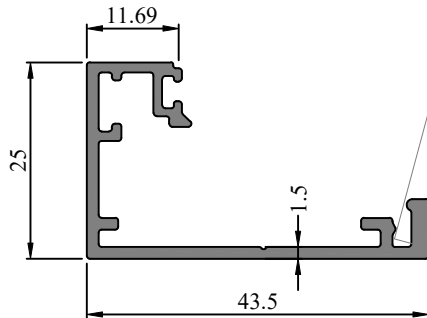
Profile Code - 366188 Weight (KG)/M - 0.435
