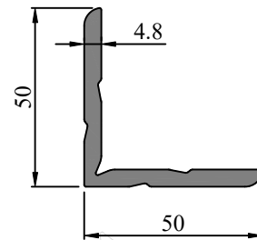
Profile Code - 421050 Weight KG /M - 1.160
