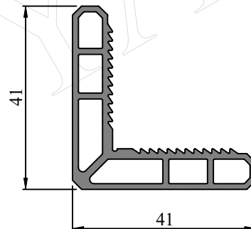
Profile Code - 481012 Weight KG /M - 0.735
