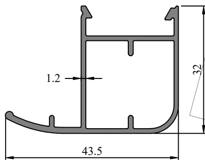
Profile Code - 431057 Weight (KG)/M - 0.463
