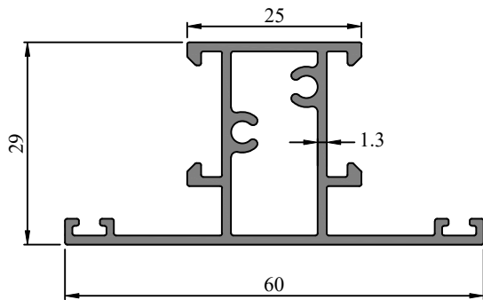
Profile Code - 366610 Weight (KG)/M - 0.650
