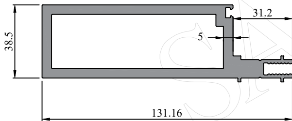
Profile Code - 273014 Weight KG /M - 4.10
