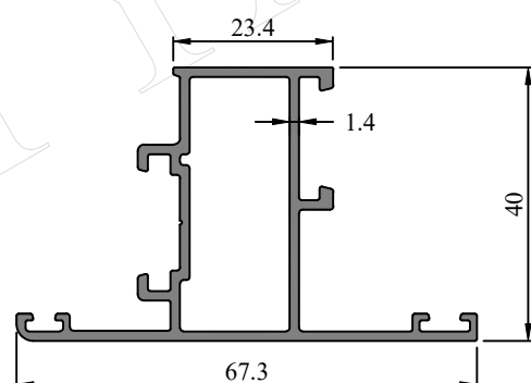
Profile Code - 366164 Weight (KG)/M - 0.778
