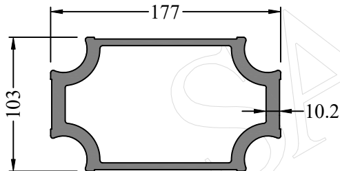
Profile Code - 3663005 Weight KG /M - 10.428
