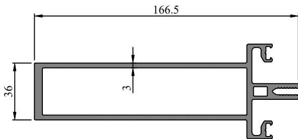
Profile Code - 272046 Weight KG /M - 3.878
