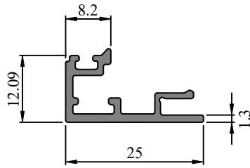
Profile Code - 366186 Weight (KG)/M - 0.214
