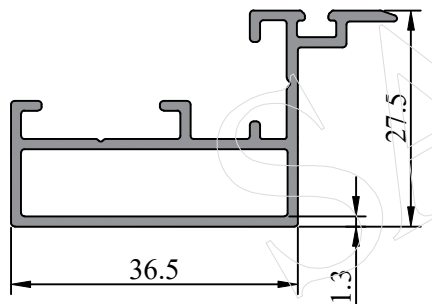
Profile Code - 541010 Weight KG /M - 0.520
