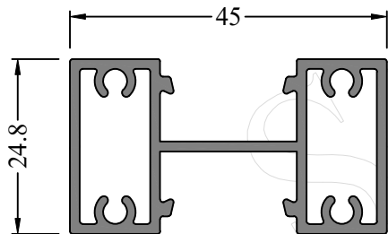
Profile Code - 366117 Weight KG /M - 0.752
