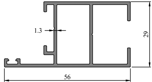
Profile Code - 366609 Weight (KG)/M - 0.622
