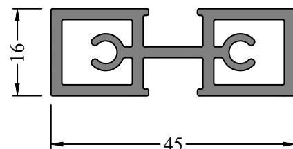
Profile Code - 366134 Weight KG /M - 0.815
