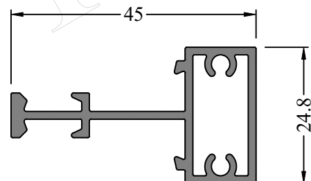
Profile Code - 366118 Weight KG /M - 0.547
