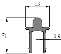
Profile Code - 366075 Weight KG /M - 0.901
