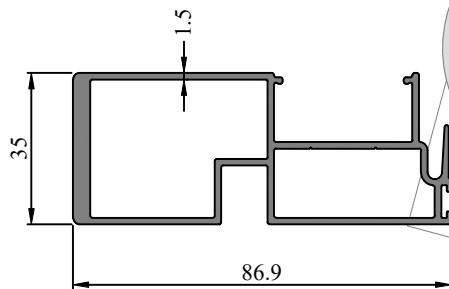
Profile Code - 366161 Weight (KG)/M - 1.428
