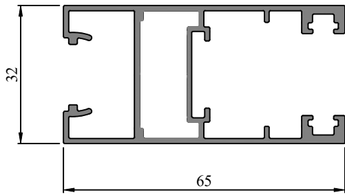
Profile Code - 366075 Weight KG /M - 0.901
