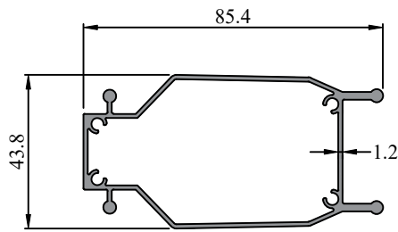
Profile Code - 447010 Weight KG /M - 1.00
