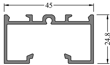
Profile Code - 366122 Weight KG /M - 0.555
