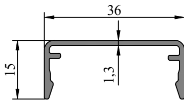
Profile Code - 366182 Weight KG /M - 0.331
