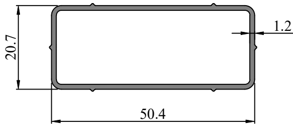
Profile Code - 353033 Weight KG /M - 0.439
