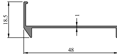
Profile Code - 431044 Weight (KG)/M - 0.210
