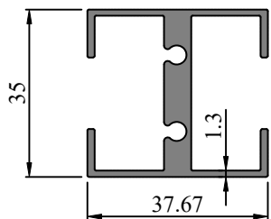
Profile Code - 363024 Weight KG /M - 0.820
