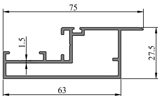
Profile Code - 541012 Weight KG /M - 0.868
