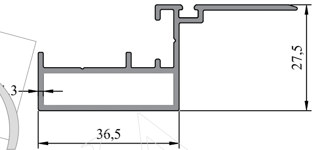
Profile Code - 542010 Weight KG /M - 0.830
