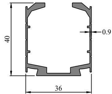
Profile Code - 366102 Weight (KG)/M - 0.604
