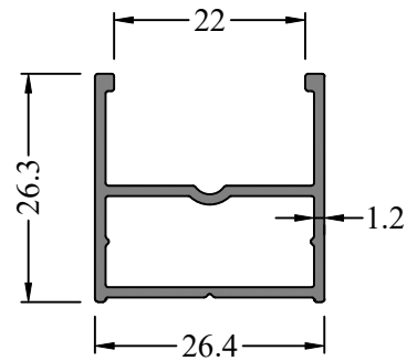
Profile Code - 366410 Weight KG /M - 0.339
