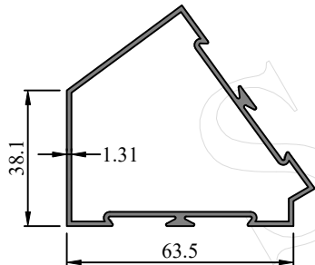
Profile Code - 404010 Weight/12' (KG) - 3.300-3.800
