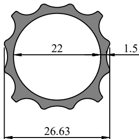
Profile Code - 335011 Weight(KG)/M - 0.464
