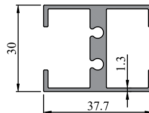
Profile Code - 363023 Weight KG /M - 0.704
