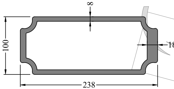
Profile Code - 3663008 Weight KG /M - 14.644
