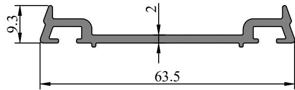
Profile Code - 366183 Weight KG /M - 0.470
