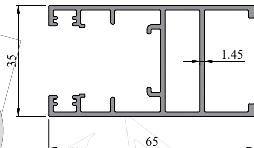
Profile Code - 363021 Weight KG /M - 0.970
