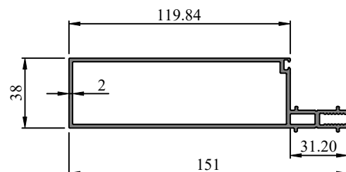
Profile Code - 273017 Weight KG /M - 2.078
