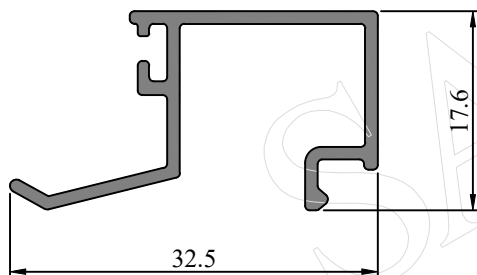
Profile Code - 245017 Weight KG /M - 0.236
