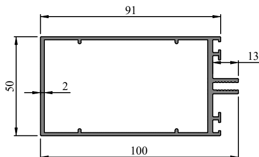
Profile Code - 271312 Weight KG /M - 1.528
