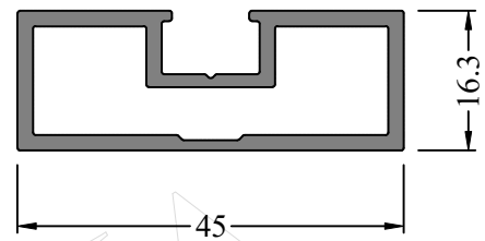
Profile Code - 366130 Weight KG /M - 0.615
