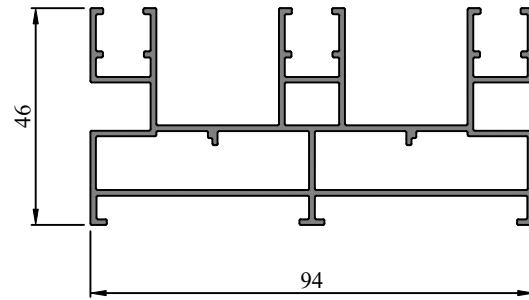
Profile Code - 366076 Weight KG /M - 1.449
