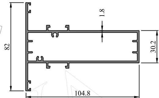
Profile Code - 366162 Weight (KG)/M - 1.872
