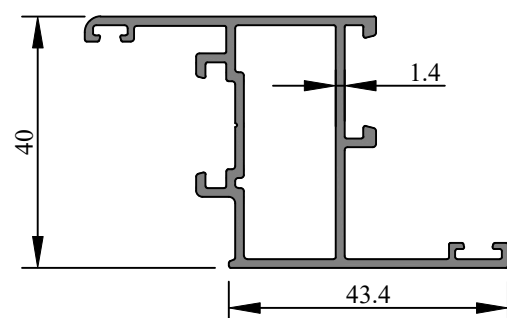
Profile Code - 366166 Weight (KG)/M - 0.766
