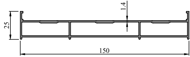
Profile Code - 366094 Weight KG /M - 1.501
