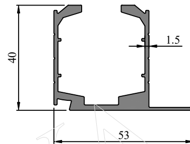
Profile Code - 366103 Weight (KG)/M - 0.993
