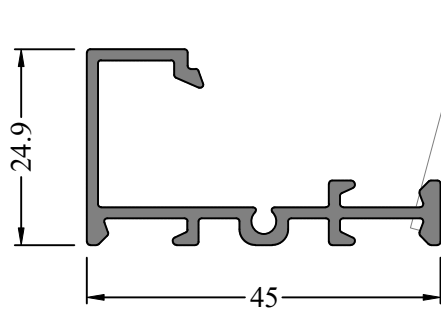
Profile Code - 366115 Weight KG /M - 0.459
