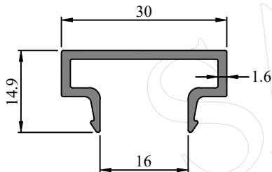
Profile Code - 431047 Weight (KG)/M - 0.279
