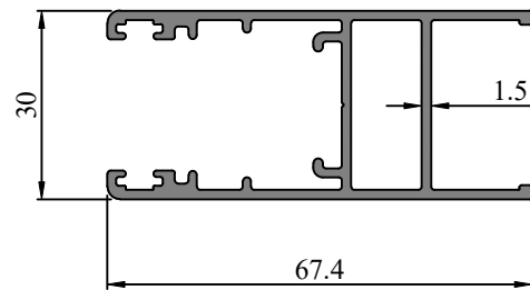
Profile Code - 363019 Weight KG /M - 0.938
