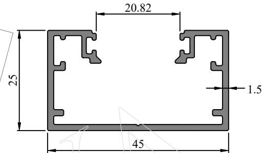
Profile Code - 366189 Weight (KG)/M - 0.574
