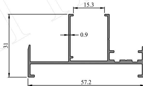
Profile Code - 431048 Weight (KG)/M - 0.445
