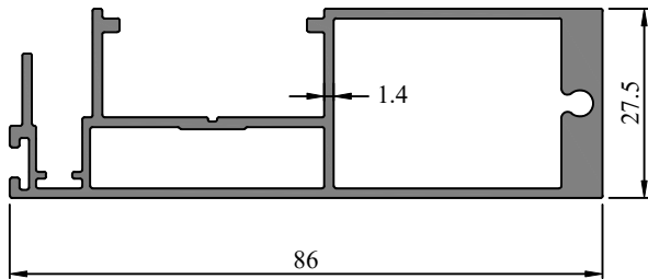
Profile Code - 366608 Weight (KG)/M - 1.282
