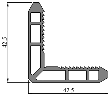
Profile Code - 481013 Weight KG /M - 0.788
