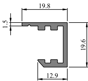
Profile Code - 431021 Weight (KG)/M - 0.264
