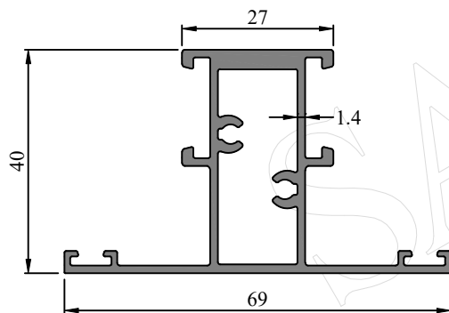
Profile Code - 366163 Weight (KG)/M - 0.932
