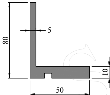
Profile Code - 321215 Weight KG /M - 2.200
