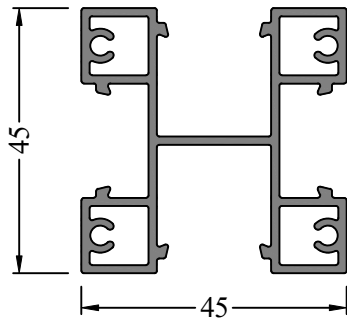
Profile Code - 366121 Weight KG /M - 1.109
