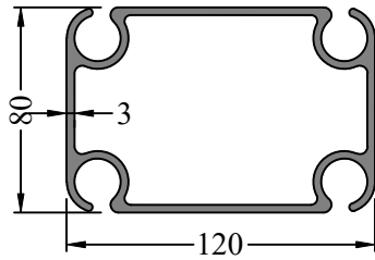
Profile Code - 3663003 Weight KG /M - 4.080
