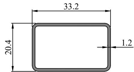
Profile Code - 353034 Weight KG /M - 0.321
