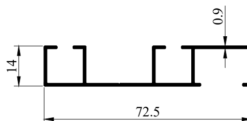
Profile Code - 366085 Weight (KG)/M - 0.377
