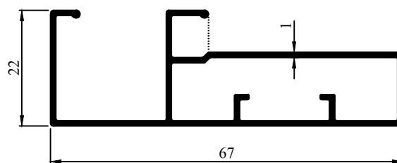
Profile Code - 366091 Weight (KG)/M - 0.516
