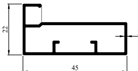
Profile Code - 366087 Weight (KG)/M - 0.386
