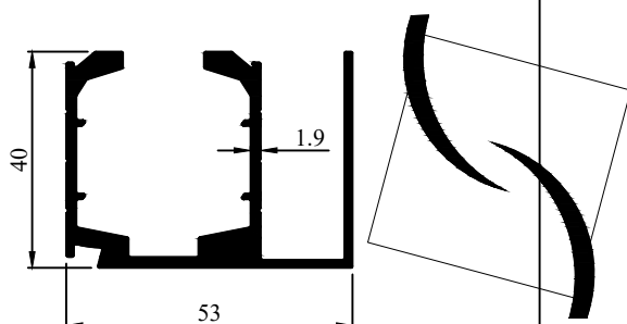
Profile Code - 366104 Weight (KG)/M - 1.165
