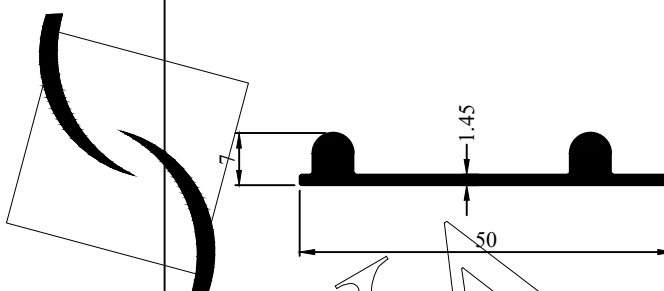
Profile Code - 452014 Weight (KG)/M - 0.343
