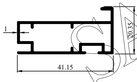
Profile Code - 366084 Weight (KG)/M - 0.381
