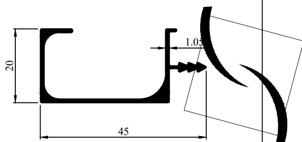
Profile Code - 366096 Weight (KG)/M - 0.321
