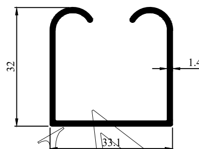
Profile Code - 366101 Weight (KG)/M - 0.420
