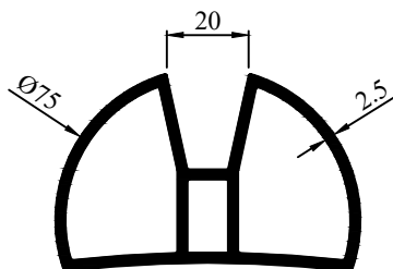
Profile Code - 431049 Weight (KG)/M - 1.887
