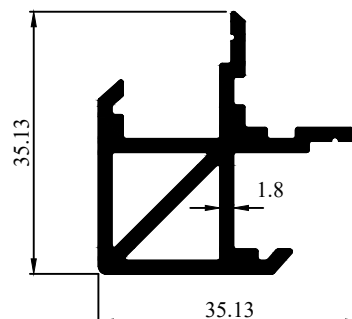
Profile Code - 431018 Weight (KG)/M - 0.721
