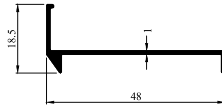
Profile Code - 431044 Weight (KG)/M - 0.210
