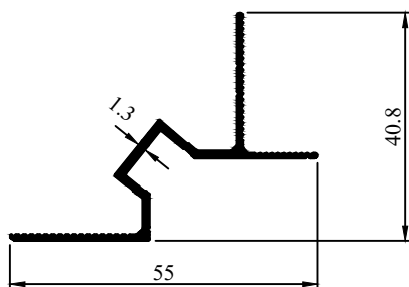
Profile Code - 431027 Weight (KG)/M - 0.335
