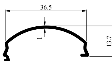
Profile Code - 431012 Weight (KG)/M - 1.291
