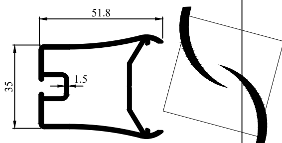
Profile Code - 431013 Weight (KG)/M - 0.791
