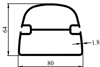
Profile Code - 431011 Weight (KG)/M - 1.668
