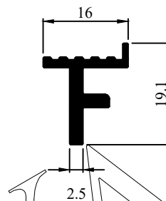
Profile Code - 431022 Weight (KG)/M - 0.214
