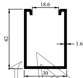
Profile Code - 431046 Weight (KG)/M - 0.529
