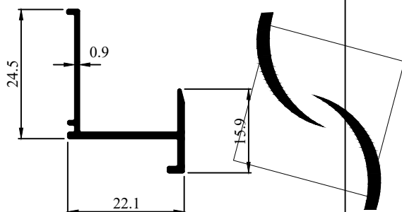
Profile Code - 431029 Weight (KG)/M - 0.186
