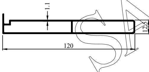
Profile Code - 431023 Weight (KG)/M - 0.828
