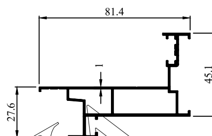
Profile Code - 431030 Weight (KG)/M - 0.822
