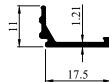
Profile Code - 431054 Weight (KG)/M - 0.106
