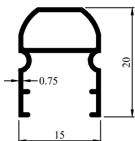
Profile Code - 431010 Weight/12' (KG) - 0.350-0.450
