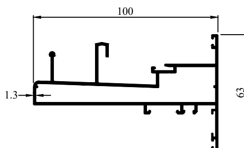
Profile Code - 431034 Weight (KG)/M - 1.352
