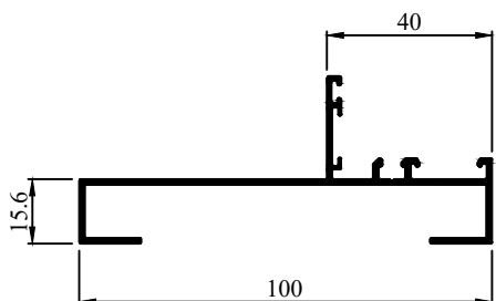
Profile Code - 431031 Weight (KG)/M - 0.209
