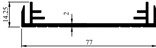
Profile Code - 431055 Weight (KG)/M - 0.548
