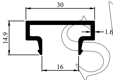
Profile Code - 431047 Weight (KG)/M - 0.279
