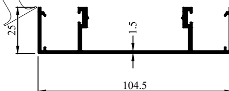
Profile Code - 431040 Weight (KG)/M - 1.016
