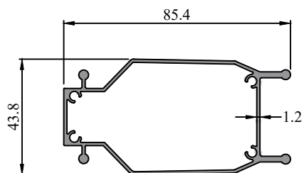
Profile Code - 447010 Weight KG / M - 1.00
