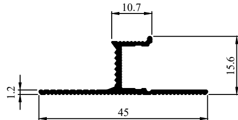
Profile Code - 431026 Weight (KG)/M - 0.212
