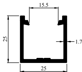
Profile Code - 431036 Weight (KG)/M - 0.389
