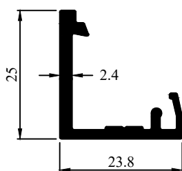
Profile Code - 431037 Weight (KG)/M - 0.341
