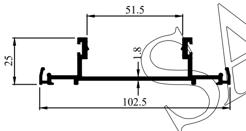
Profile Code - 431039 Weight (KG)/M - 0.924
