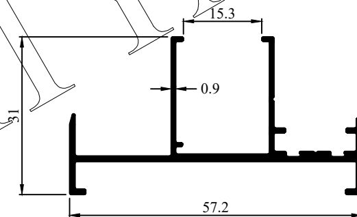
Profile Code - 431048 Weight (KG)/M - 0.445
