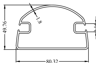
Profile Code - 431012 Weight (KG)/M - 1.291
