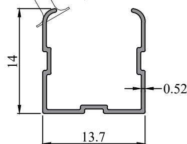
Profile Code - 404014 Weight (KG)/M - 0.062
