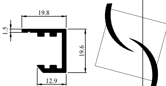
Profile Code - 431021 Weight (KG)/M - 0.264
