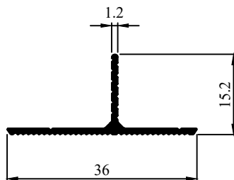
Profile Code - 431025 Weight (KG)/M - 0.146
