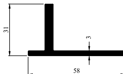
Profile Code - 431042 Weight (KG)/M - 0.847
