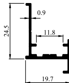
Profile Code - 431028 Weight (KG)/M - 0.198
