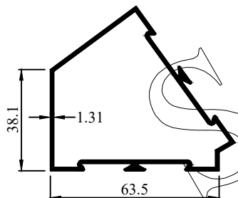
Profile Code - 404010 Weight/12' (KG) - 3.300-3.800
