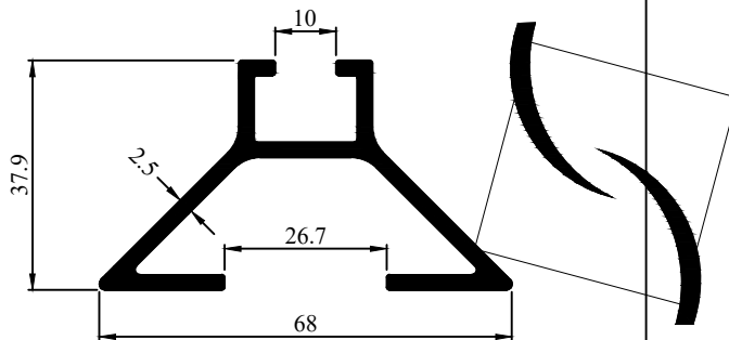
Profile Code - 431045 Weight (KG)/M - 1.052
