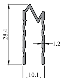
Profile Code - 422010 Weight KG / M - 0.180
