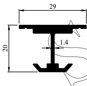
Profile Code - 431015 Weight (KG)/M - 0.355
