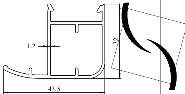
Profile Code - 431057 Weight (KG)/M - 0.463
