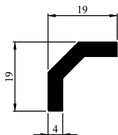
Profile Code - 431035 Weight (KG)/M - 0.321
