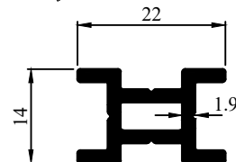
Profile Code - 431024 Weight (KG)/M - 0.327
