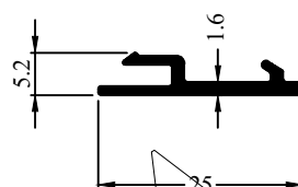
Profile Code - 431038 Weight (KG)/M - 0.136
