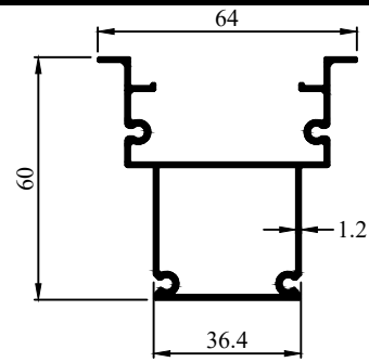
Profile Code - 431056 Weight (KG)/M - 0.884
