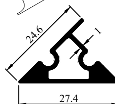
Profile Code - 431032 Weight (KG)/M - 0.280
