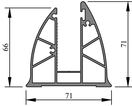
Profile Code - 366211 Weight KG /M - 2.309
