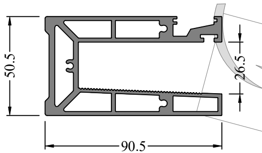
Profile Code - 366213 Weight KG /M - 3.160
