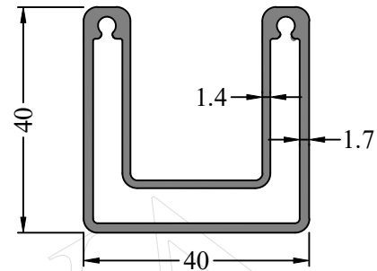
Profile Code - 366215 Weight KG /M - 0.943
