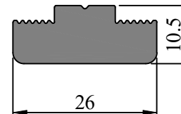
SEC. NO. 452027 WEIGHT - 0.664 Kg/M
