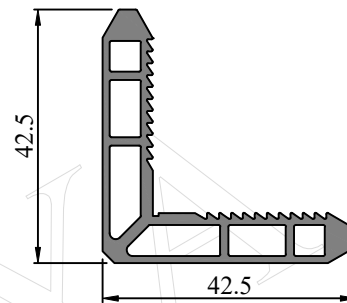
SEC. NO. 452017 WEIGHT - 0.523 Kg/M
