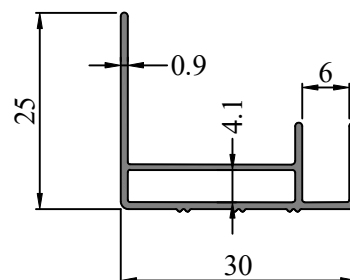
SEC. NO. IS00240 WEIGHT - 0.222 Kg/M
