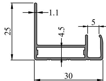
SEC. NO. IS00144 WEIGHT - 0.270 Kg/M
