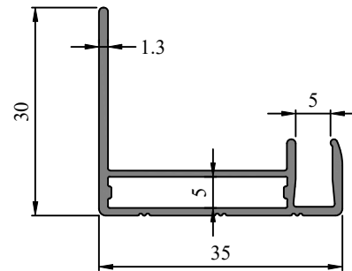
SEC. NO. IS0053 WEIGHT - 0.330 Kg/M
