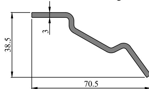
SEC. NO. IS00245 WEIGHT - 0.692 Kg/M
