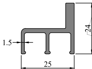
SEC. NO. IS0012 WEIGHT - 0.395 Kg/M
