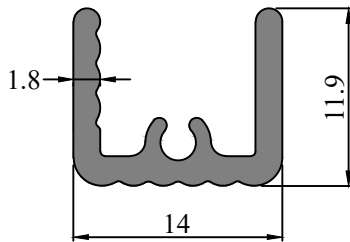
SEC. NO. IS0010 WEIGHT - 0.175 Kg/M
