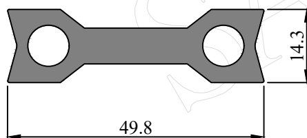
SEC. NO. IS0062 WEIGHT - 1.10 Kg/M
