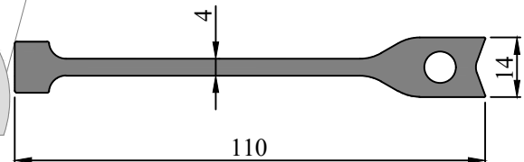
SEC. NO. IS00243 WEIGHT - 1.822 Kg/M
