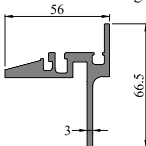
SEC. NO. IS00121 WEIGHT - 1.550 Kg/M
