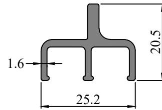
SEC. NO. IS0011 WEIGHT - 0.330 Kg/M
