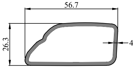
SEC. NO. IS00224 WEIGHT - 0.756 Kg/M
