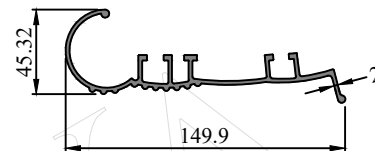
SEC. NO. IS0061 WEIGHT - 1.80 Kg/M
