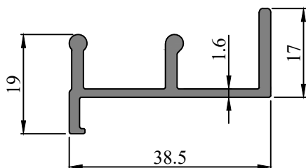
SEC. NO. IS00260 WEIGHT - 0.434 Kg/M
