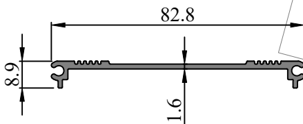
SEC. NO. IS00270 WEIGHT - 0.493 Kg/M
