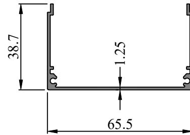
SEC. NO. IS00221 WEIGHT - 0.570 Kg/M
