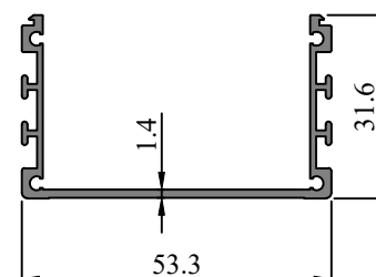
SEC. NO. IS00154R1 WEIGHT - 0.500 Kg/M
