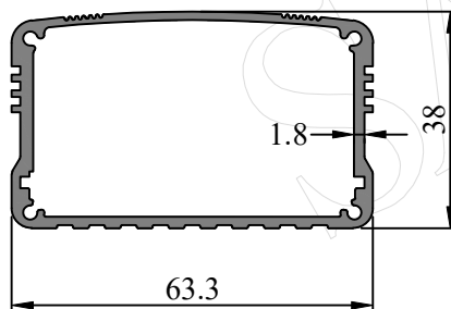
SEC. NO. IS00153 WEIGHT - 0.110 Kg/M
