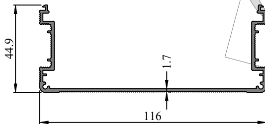
SEC. NO. IS00146 WEIGHT - 1.00 Kg/M
