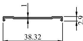
SEC. NO. IS00153 WEIGHT - 0.110 Kg/M
