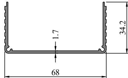
SEC. NO. IS0002 WEIGHT - 0.640 Kg/M
