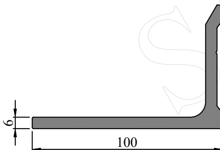
SEC. NO. FW0041 WEIGHT - 2.640 Kg/M
