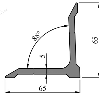
SEC. NO. IS00210 WEIGHT - 1.71 Kg/M
