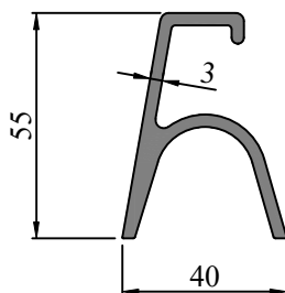
SEC. NO. IS0019 WEIGHT - 1.10 Kg/M
