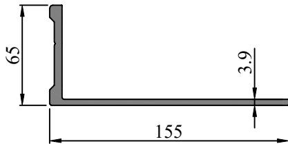
SEC. NO. FW0008 WEIGHT - 3.117 Kg/M
