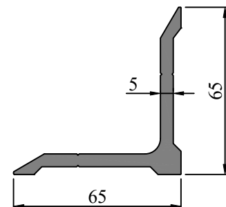
SEC. NO. IS0041 WEIGHT - 1.70 Kg/M
