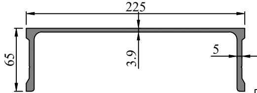
SEC. NO. FW0037 WEIGHT - 4.898 Kg/M
