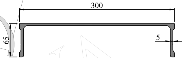
SEC. NO. FW0019 WEIGHT - 5.161 Kg/M
