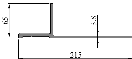
SEC. NO. FW0065 WEIGHT - 3.232 Kg/M
