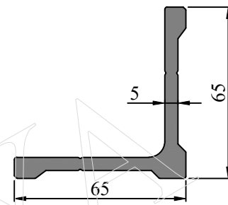
SEC. NO. FW0022 WEIGHT - 1.942 Kg/M
