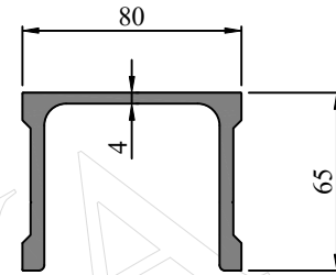
SEC. NO. IS00192 WEIGHT - 2.88 Kg/M
