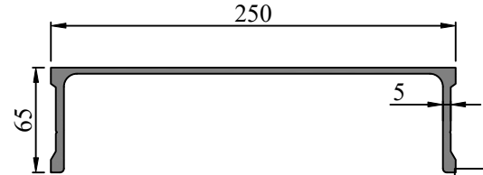
SEC. NO. FW0018 WEIGHT - 4.635 Kg/M
