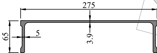
SEC. NO. FW0037 WEIGHT - 4.898 Kg/M
