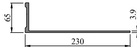
SEC. NO. FW0009 WEIGHT - 3.380 Kg/M
