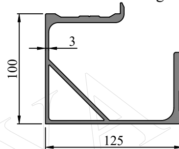
SEC. NO. FW0054 WEIGHT - 4.752 Kg/M
