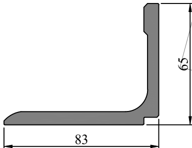
SEC. NO. IS00209 WEIGHT - 1.24 Kg/M
