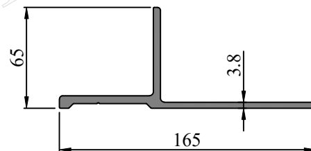
SEC. NO. FW0066 WEIGHT - 3.744 Kg/M
