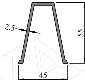
SEC. NO. IS0059 WEIGHT - 0.880 Kg/M
