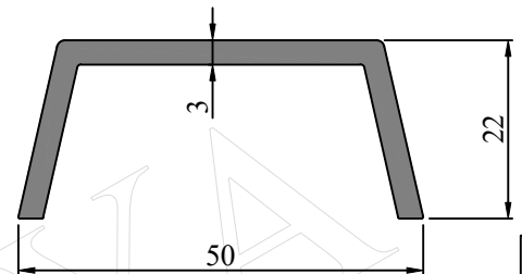
SEC. NO. IS0018 WEIGHT - 1.10 Kg/M
