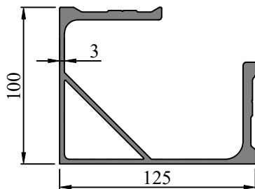
SEC. NO. FW0055 WEIGHT - 4.550 Kg/M
