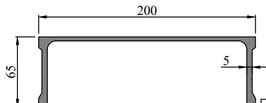
SEC. NO. FW0017 WEIGHT - 4.108 Kg/M
