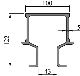
SEC. NO. FW0057 WEIGHT - 5.450 Kg/M
