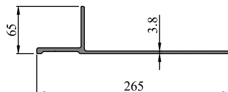
SEC. NO. FW0066 WEIGHT - 3.744 Kg/M
