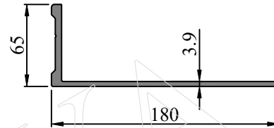
SEC. NO. FW0031 WEIGHT - 2.853 Kg/M
