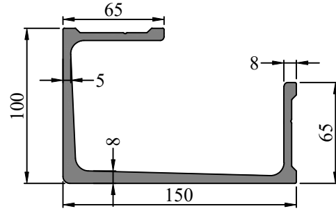
SEC. NO. FW0028 WEIGHT - 6.160 Kg/M
