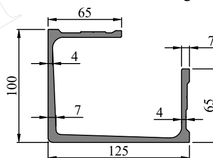
SEC. NO. FW0028 WEIGHT - 6.160 Kg/M
