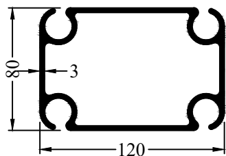
Profile Code - 3663003 Weight KG /M - 4.080
