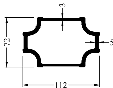
Profile Code - 3663027 Weight KG /M - 3.748
