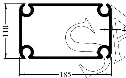
Profile Code - 3663004 Weight KG /M - 7.766
