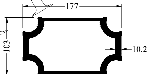
Profile Code - 3663008 Weight KG /M - 14.644
