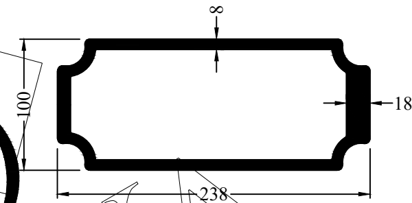
Profile Code - 3663008 Weight KG /M - 14.644
