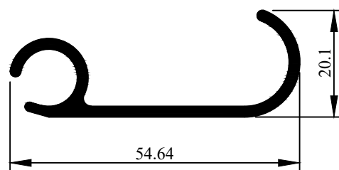
Profile Code - 3663002 Weight KG /M - 0.511
