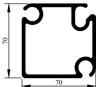
Profile Code - 3663001 Weight KG /M - 2.723
