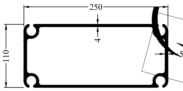
Profile Code - 3663006 Weight KG /M - 9.275
