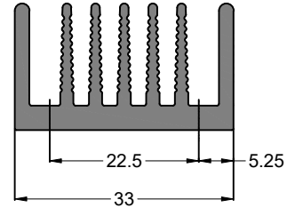
SEC. NO. IS00269 WEIGHT - 1.633 Kg/M
