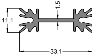
SEC. NO. IS00212 WEIGHT - 0.340 Kg/M
