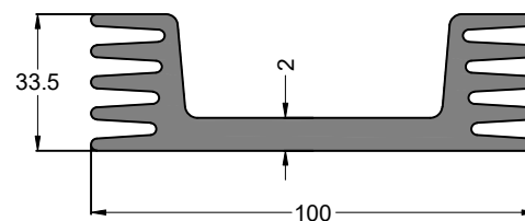
SEC. NO. IS00308 WEIGHT - 3.998 Kg/M
