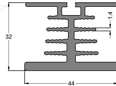
SEC. NO. IS00308 WEIGHT - 3.998 Kg/M
