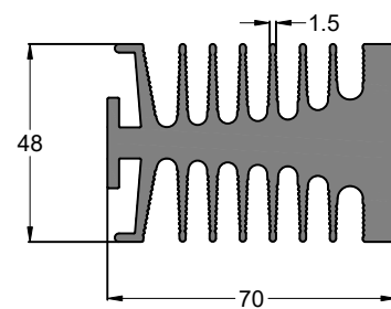
SEC. NO. IS00287 WEIGHT - 4.617 Kg/M
