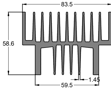
SEC. NO. IS00288 WEIGHT - 4.736 Kg/M
