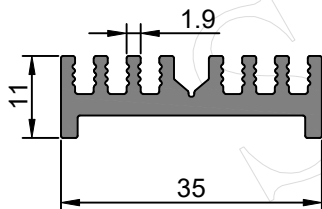
SEC. NO. IS00282 WEIGHT - 0.513 Kg/M
