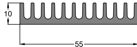
SEC. NO. IS00202 WEIGHT - 1.33 Kg/M
