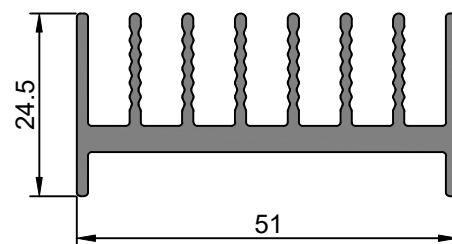
SEC. NO. IS00285 WEIGHT - 0.961 Kg/M
