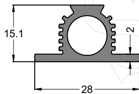
SEC. NO. IS00307 WEIGHT - 4.154 Kg/M
