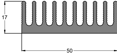
SEC. NO. IS0064 WEIGHT - 1.20 Kg/M
