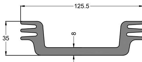
SEC. NO. IS00307 WEIGHT - 4.154 Kg/M
