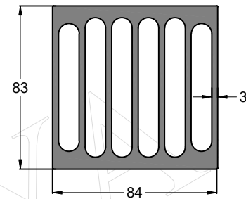
SEC. NO. IS00293 WEIGHT - 1.245 Kg/M
