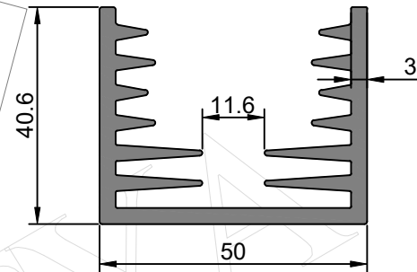
SEC. NO. IS00283 WEIGHT - 0.287 Kg/M
