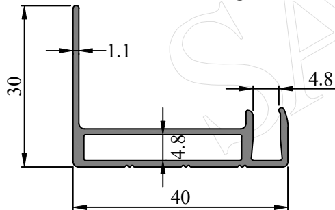
SEC. NO. IS0093 WEIGHT - 0.390 Kg/M
