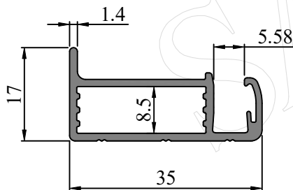
SEC. NO. IS0091 WEIGHT - 0.320 Kg/M
