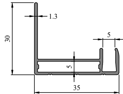
SEC. NO. IS0053 WEIGHT - 0.330 Kg/M
