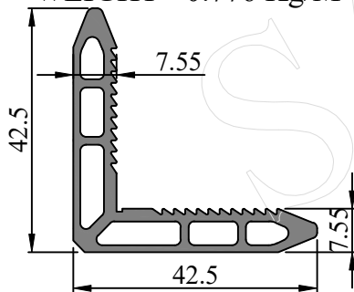
SEC. NO. SL0003 WEIGHT - 0.776 Kg/M
