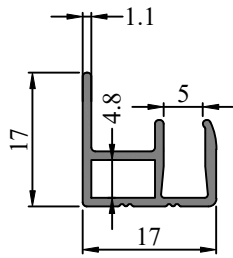
SEC. NO. IS0094 WEIGHT - 0.180 Kg/M
