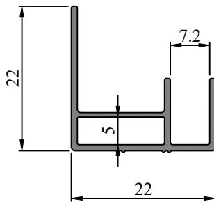
SEC. NO. IS00216 WEIGHT - 0.180 Kg/M
