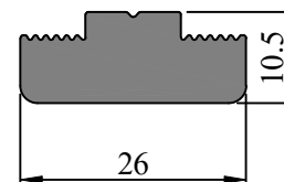
SEC. NO. 452027 WEIGHT - 0.664 Kg/M
