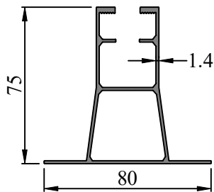
SEC. NO. 452019 R1 WEIGHT - 1.185 Kg/M
