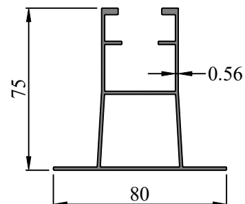
SEC. NO. 452019 WEIGHT - 1.142 Kg/M
