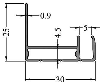
SEC. NO. IS00111 WEIGHT - 0.240 Kg/M
