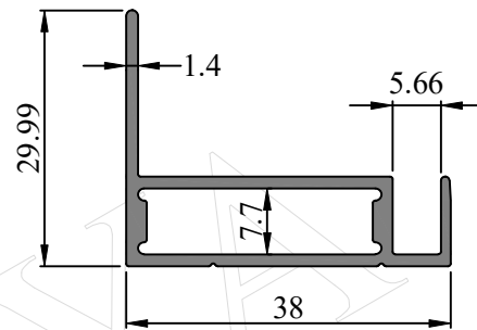
SEC. NO. 414010 WEIGHT - 0.445 Kg/M
