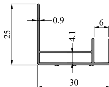
SEC. NO. IS00240 WEIGHT - 0.222 Kg/M
