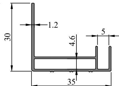
SEC. NO. IS00215 WEIGHT - 0.318 Kg/M
