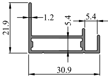
SEC. NO. 415010 WEIGHT - 0.270 Kg/M
