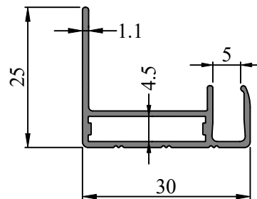
SEC. NO. IS00144 WEIGHT - 0.270 Kg/M
