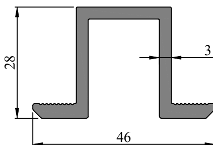
SEC. NO. 452018 WEIGHT - 0.798 Kg/M
