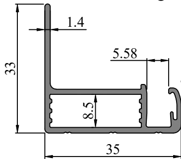
SEC. NO. IS00247 WEIGHT - 0.423 Kg/M
