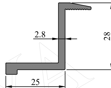
SEC. NO. 452021 WEIGHT - 0.467 Kg/M
