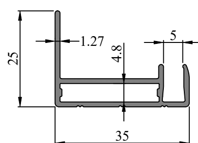
SEC. NO. IS0092 WEIGHT - 0.350 Kg/M
