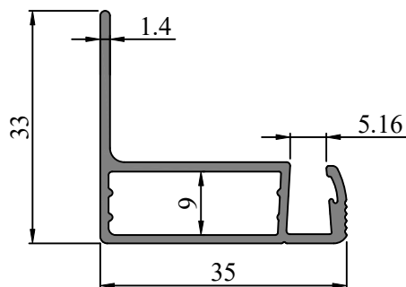
SEC. NO. IS00238 WEIGHT - 0.403 Kg/M
