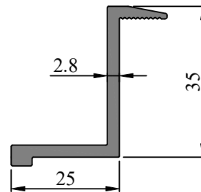
SEC. NO. 452019 WEIGHT - 1.142 Kg/M
