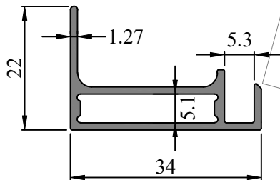
SEC. NO. 413009 WEIGHT - 0.340 Kg/M
