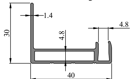
SEC. NO. IS0050 WEIGHT - 0.410 Kg/M
