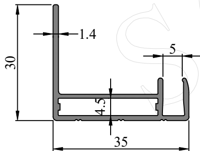
SEC. NO. IS00143 WEIGHT - 0.365 Kg/M
