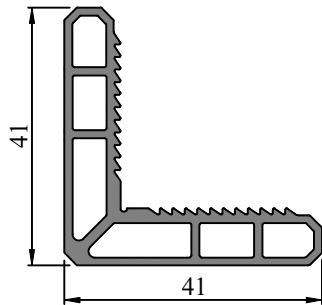
SEC. NO. 481012 WEIGHT - 0.735 Kg/M
