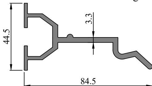
SEC. NO. 452026 WEIGHT - 1.290 Kg/M
