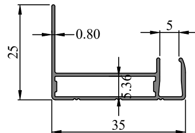
SEC. NO. IS0092 WEIGHT - 0.350 Kg/M
