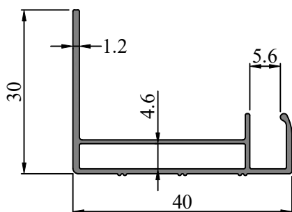
SEC. NO. IS00214 WEIGHT - 0.339 Kg/M
