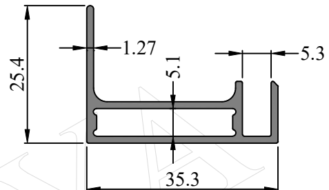
SEC. NO. 412009 WEIGHT - 0.380 Kg/M
