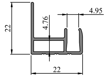
SEC. NO. IS0090 WEIGHT - 0.230 Kg/M
