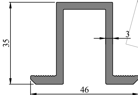
SEC. NO. 452023 WEIGHT - 0.912 Kg/M
