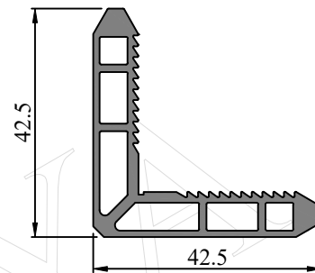
SEC. NO. 452017 WEIGHT - 0.523 Kg/M
