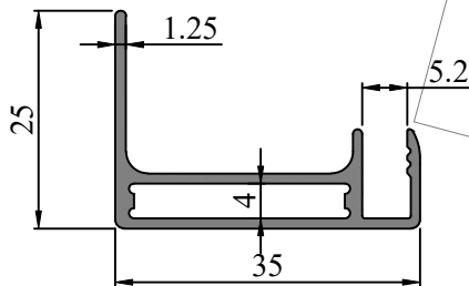
SEC. NO. IS00143 WEIGHT - 0.365 Kg/M
