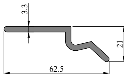
SEC. NO. 452027 WEIGHT - 0.664 Kg/M
