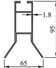
SEC. NO. 452021 WEIGHT - 0.467 Kg/M
