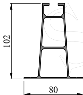
SEC. NO. 452024 WEIGHT - 1.876 Kg/M
