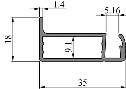
SEC. NO. IS00239 WEIGHT - 0.322 Kg/M
