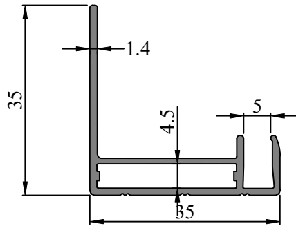
SEC. NO. IS00145 WEIGHT - 0.380 Kg/M
