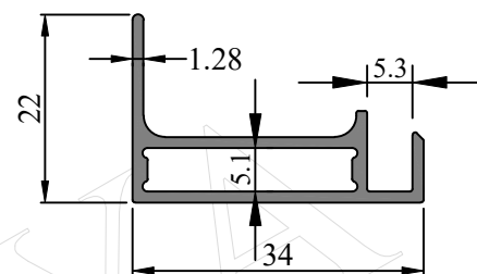
SEC. NO. 413010 WEIGHT - 0.345 Kg/M
