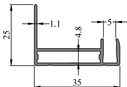
SEC. NO. IS0091 WEIGHT - 0.320 Kg/M
