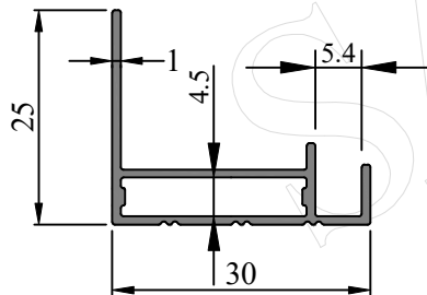
SEC. NO. IS00150 WEIGHT - 0.240 Kg/M
