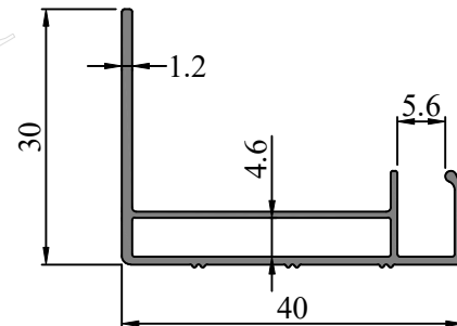
SEC. NO. IS00173 WEIGHT - 0.300 Kg/M
